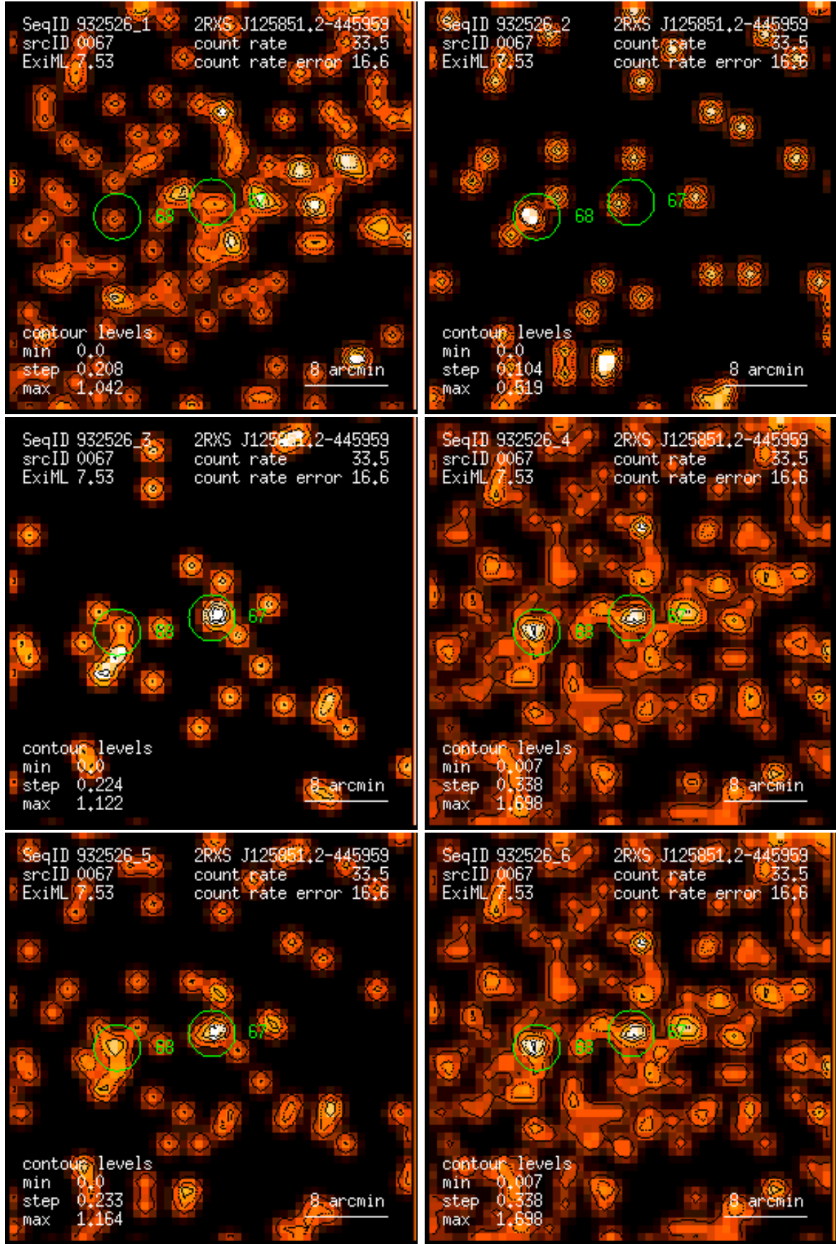
Figure 67: RASS 932526: detection 0067: band rate images, Gaussian filter: (1) PSPC channels 11 – 41, (2) 52 – 90, (3) 91 – 201, (4) 11 – 235, (5) 52 – 201, (6) 11 – 201. Broad band rates in counts/ks. Band rate contour levels in counts/ks/arcmin 2 .
