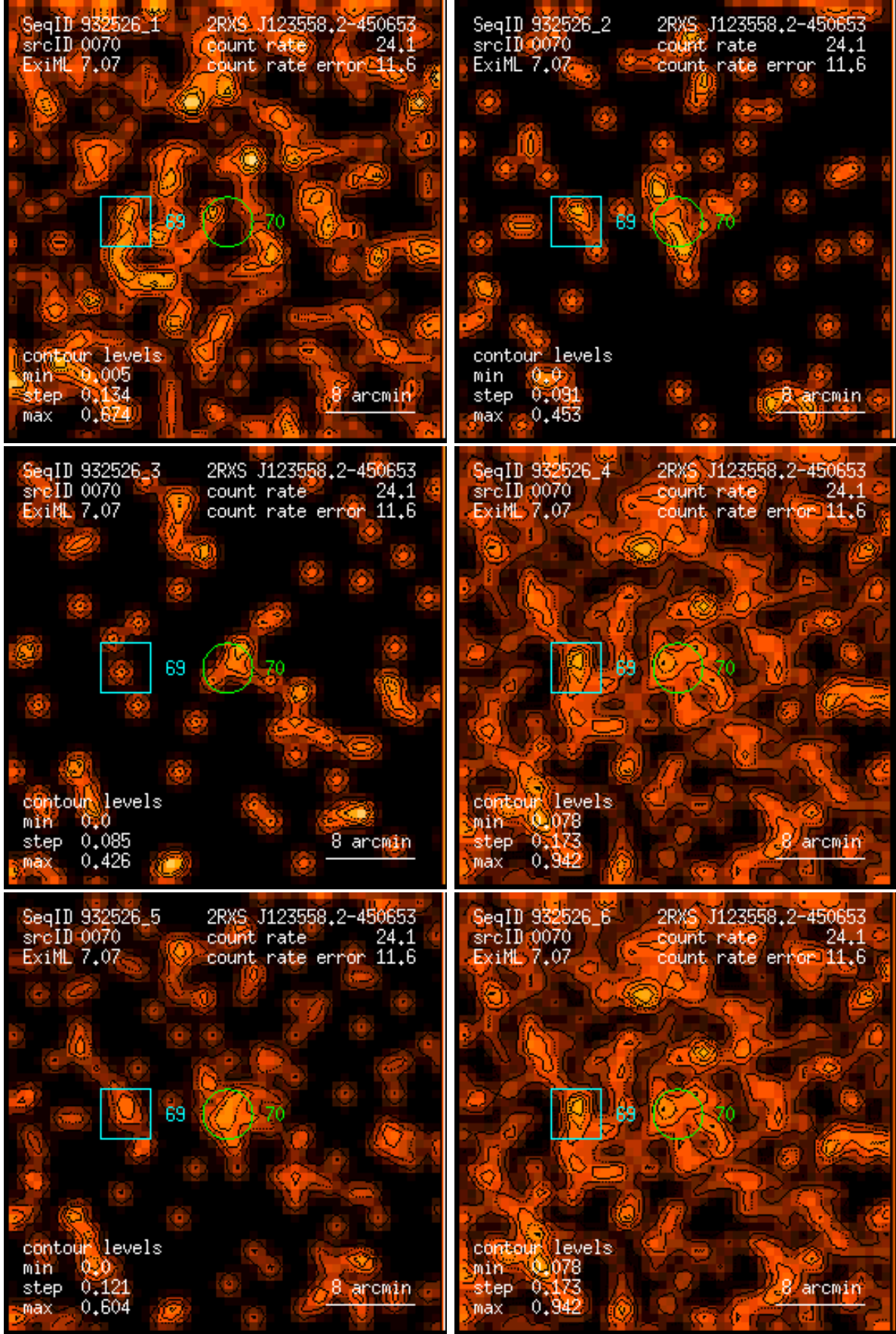
Figure 70: RASS 932526: detection 0070: band rate images, Gaussian filter: (1) PSPC channels 11 – 41, (2) 52 – 90, (3) 91 – 201, (4) 11 – 235, (5) 52 – 201, (6) 11 – 201. Broad band rates in counts/ks. Band rate contour levels in counts/ks/arcmin 2 .
