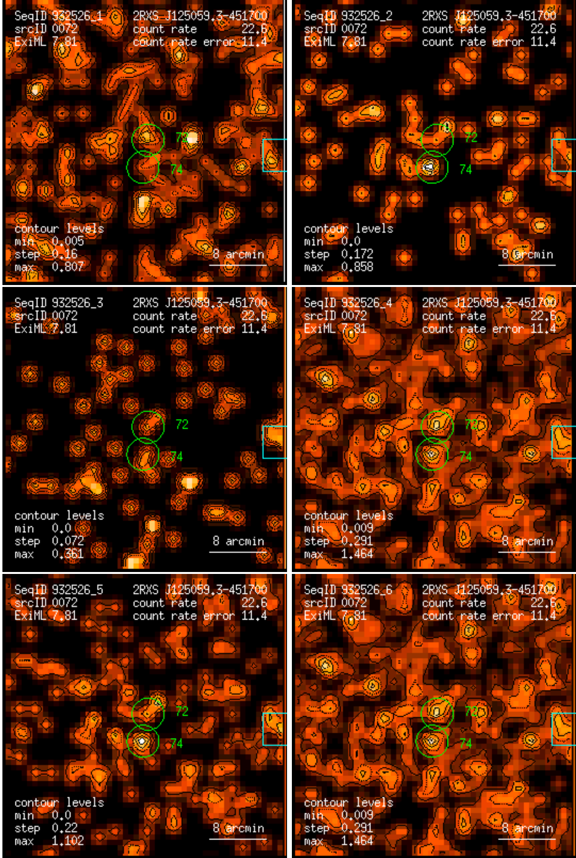
Figure 72: RASS 932526: detection 0072: band rate images, Gaussian filter: (1) PSPC channels 11 – 41, (2) 52 – 90, (3) 91 – 201, (4) 11 – 235, (5) 52 – 201, (6) 11 – 201. Broad band rates in counts/ks. Band rate contour levels in counts/ks/arcmin 2 .
