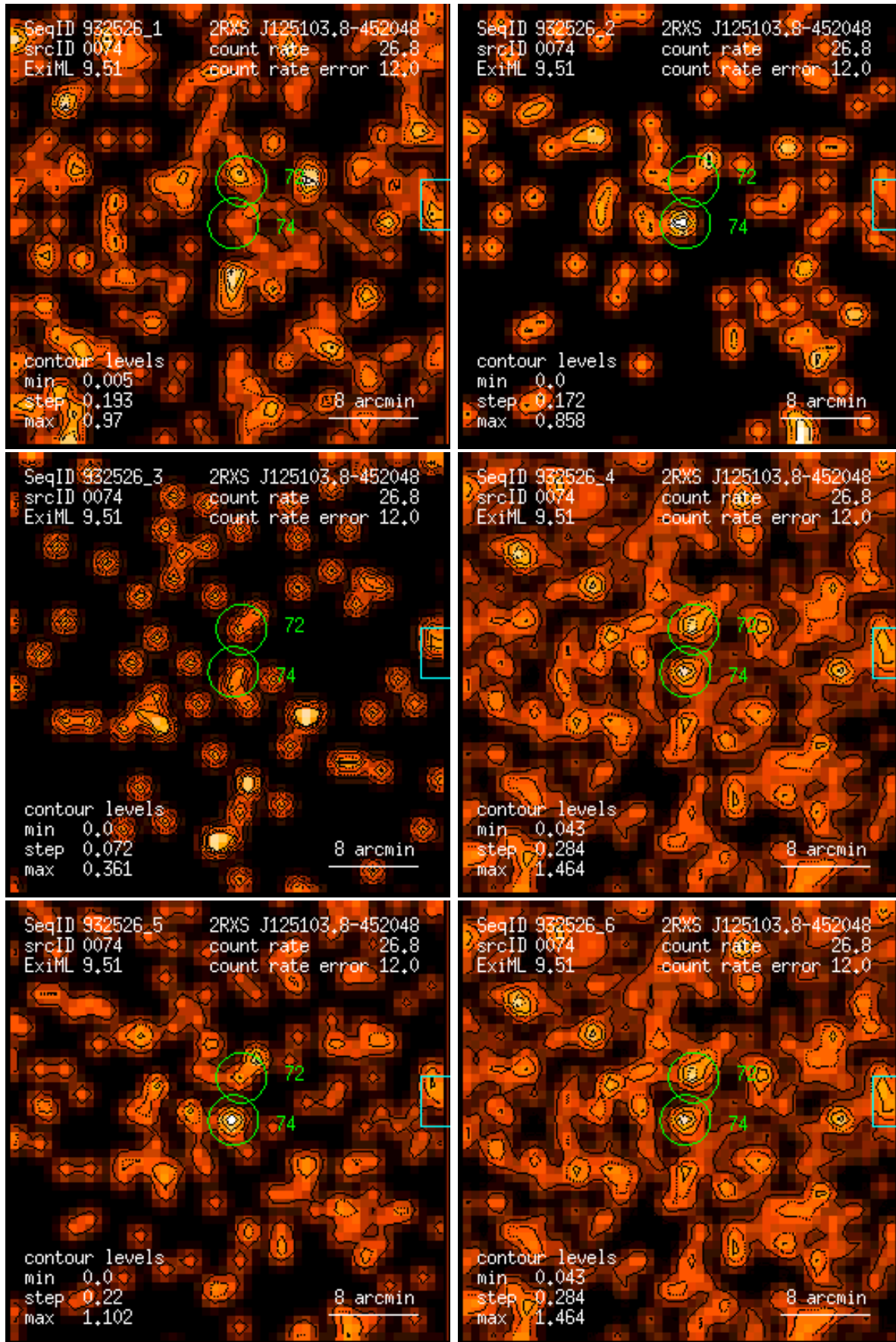
Figure 74: RASS 932526: detection 0074: band rate images, Gaussian filter: (1) PSPC channels 11 – 41, (2) 52 – 90, (3) 91 – 201, (4) 11 – 235, (5) 52 – 201, (6) 11 – 201. Broad band rates in counts/ks. Band rate contour levels in counts/ks/arcmin 2 .
