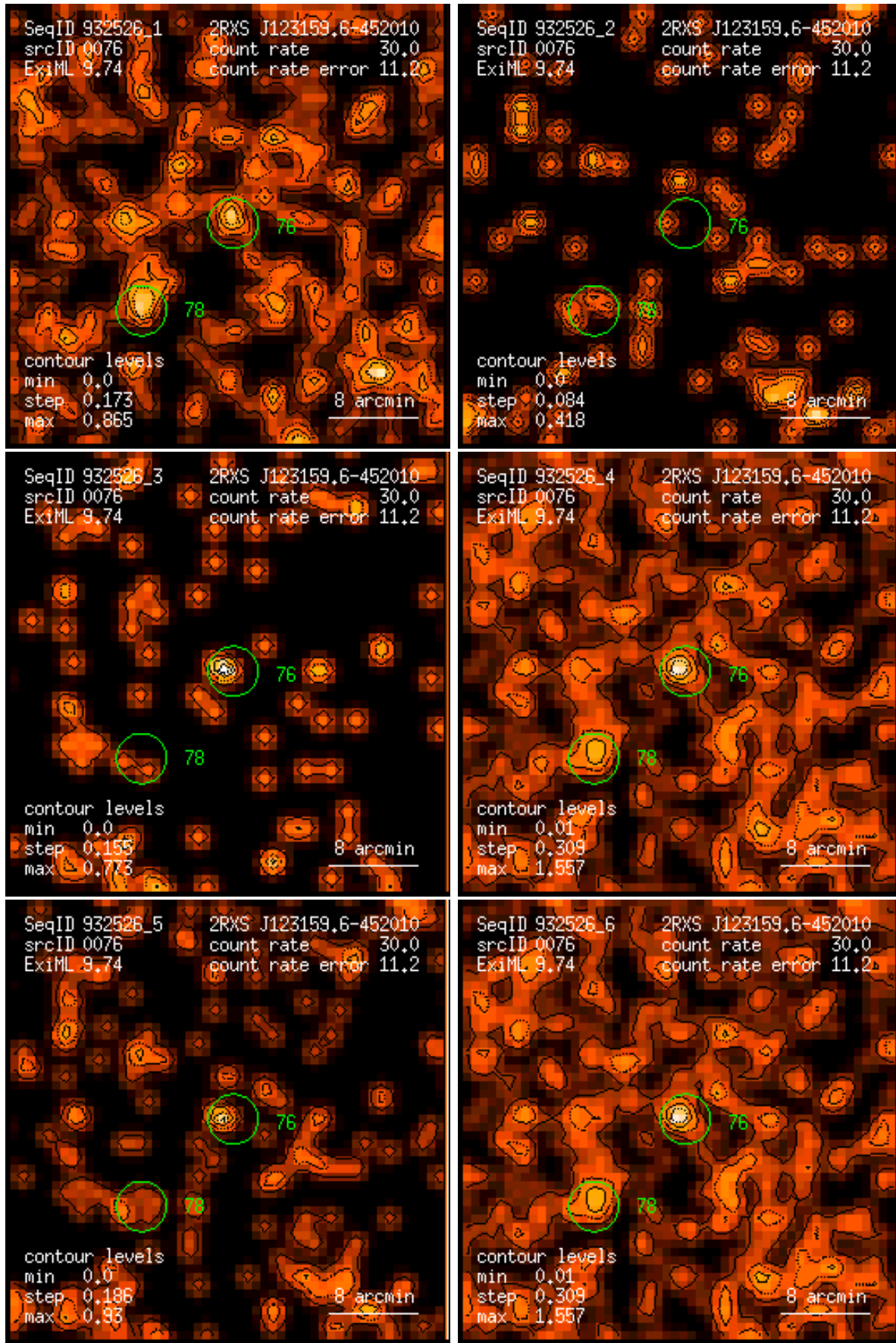
Figure 76: RASS 932526: detection 0076: band rate images, Gaussian filter: (1) PSPC channels 11 – 41, (2) 52 – 90, (3) 91 – 201, (4) 11 – 235, (5) 52 – 201, (6) 11 – 201. Broad band rates in counts/ks. Band rate contour levels in counts/ks/arcmin 2 .
