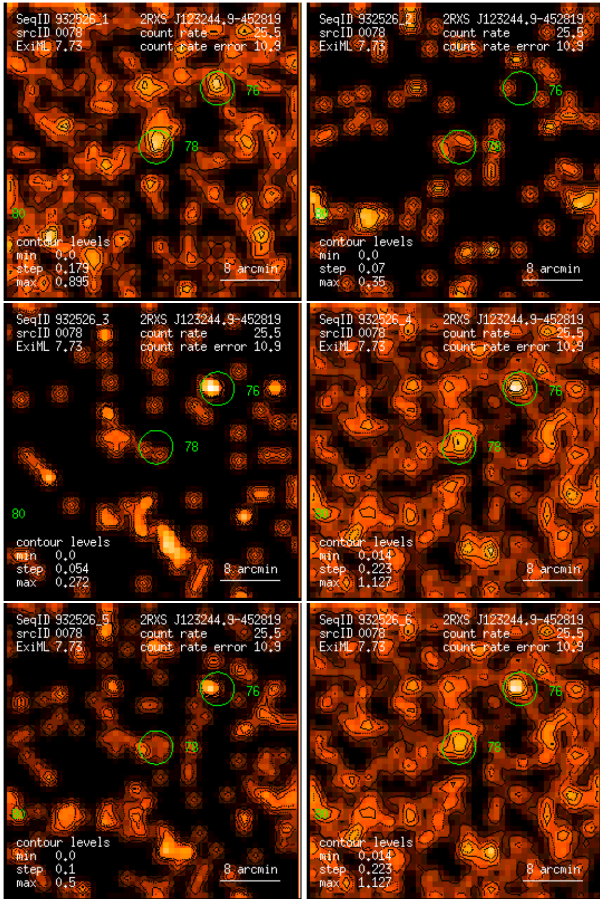
Figure 78: RASS 932526: detection 0078: band rate images, Gaussian filter: (1) PSPC channels 11 – 41, (2) 52 – 90, (3) 91 – 201, (4) 11 – 235, (5) 52 – 201, (6) 11 – 201. Broad band rates in counts/ks. Band rate contour levels in counts/ks/arcmin 2 .
