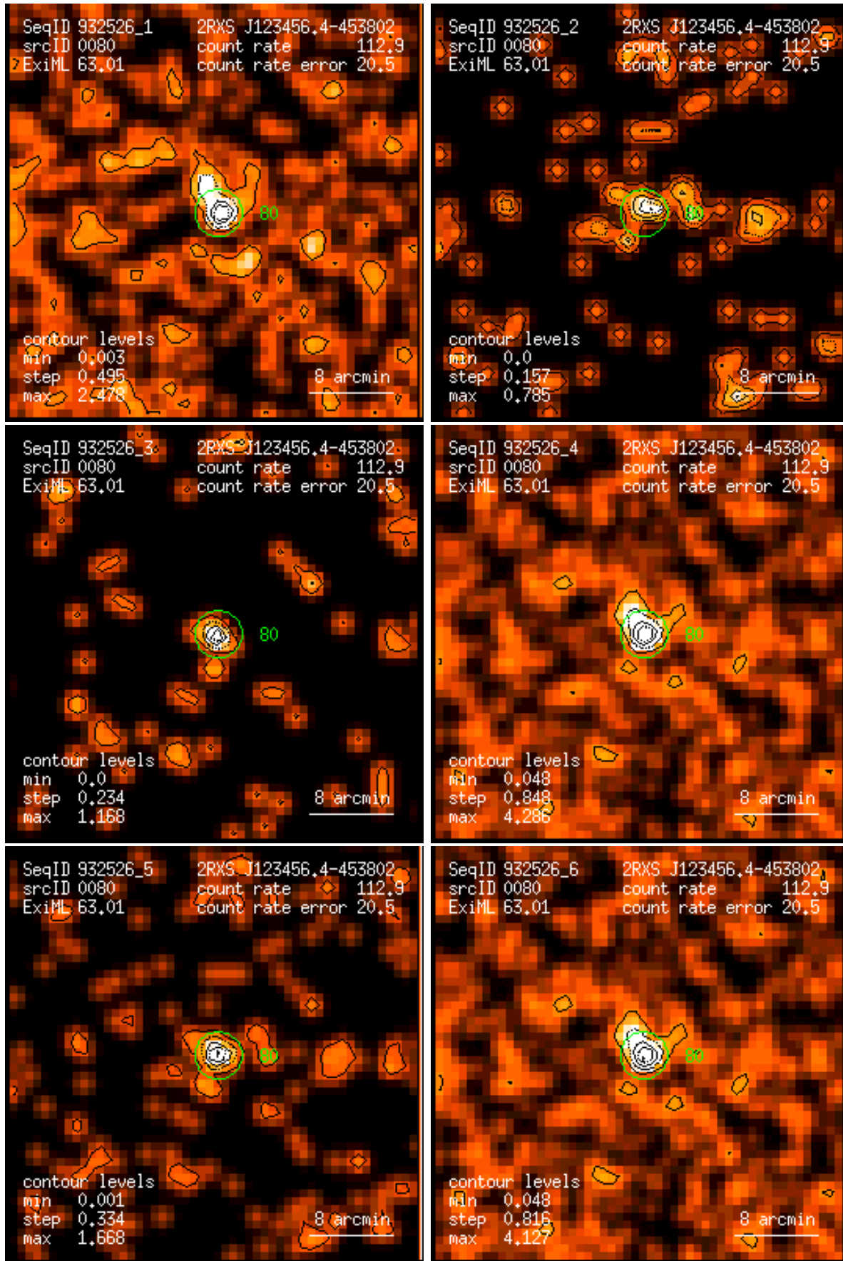
Figure 80: RASS 932526: detection 0080: band rate images, Gaussian filter: (1) PSPC channels 11 – 41, (2) 52 – 90, (3) 91 – 201, (4) 11 – 235, (5) 52 – 201, (6) 11 – 201. Broad band rates in counts/ks. Band rate contour levels in counts/ks/arcmin 2 .
