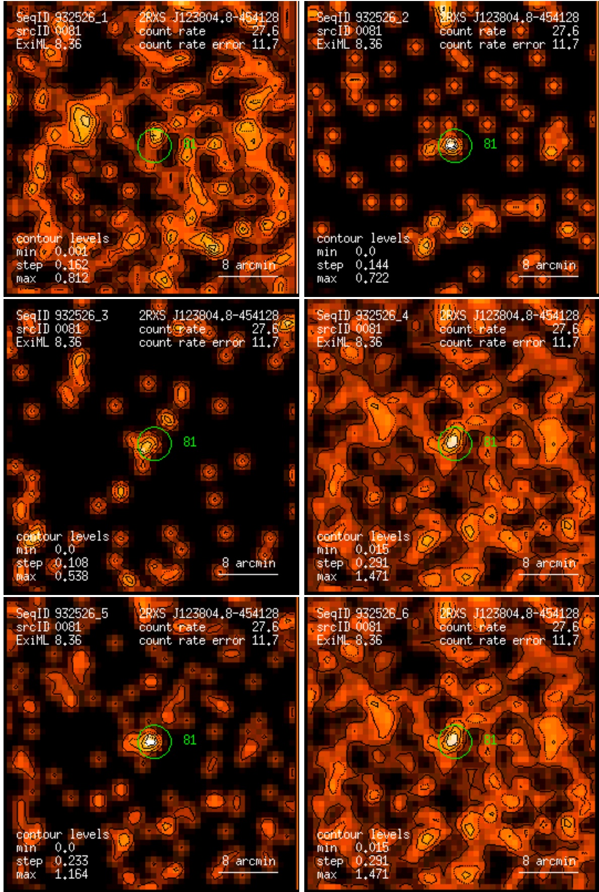
Figure 81: RASS 932526: detection 0081: band rate images, Gaussian filter: (1) PSPC channels 11 – 41, (2) 52 – 90, (3) 91 – 201, (4) 11 – 235, (5) 52 – 201, (6) 11 – 201. Broad band rates in counts/ks. Band rate contour levels in counts/ks/arcmin 2 .
