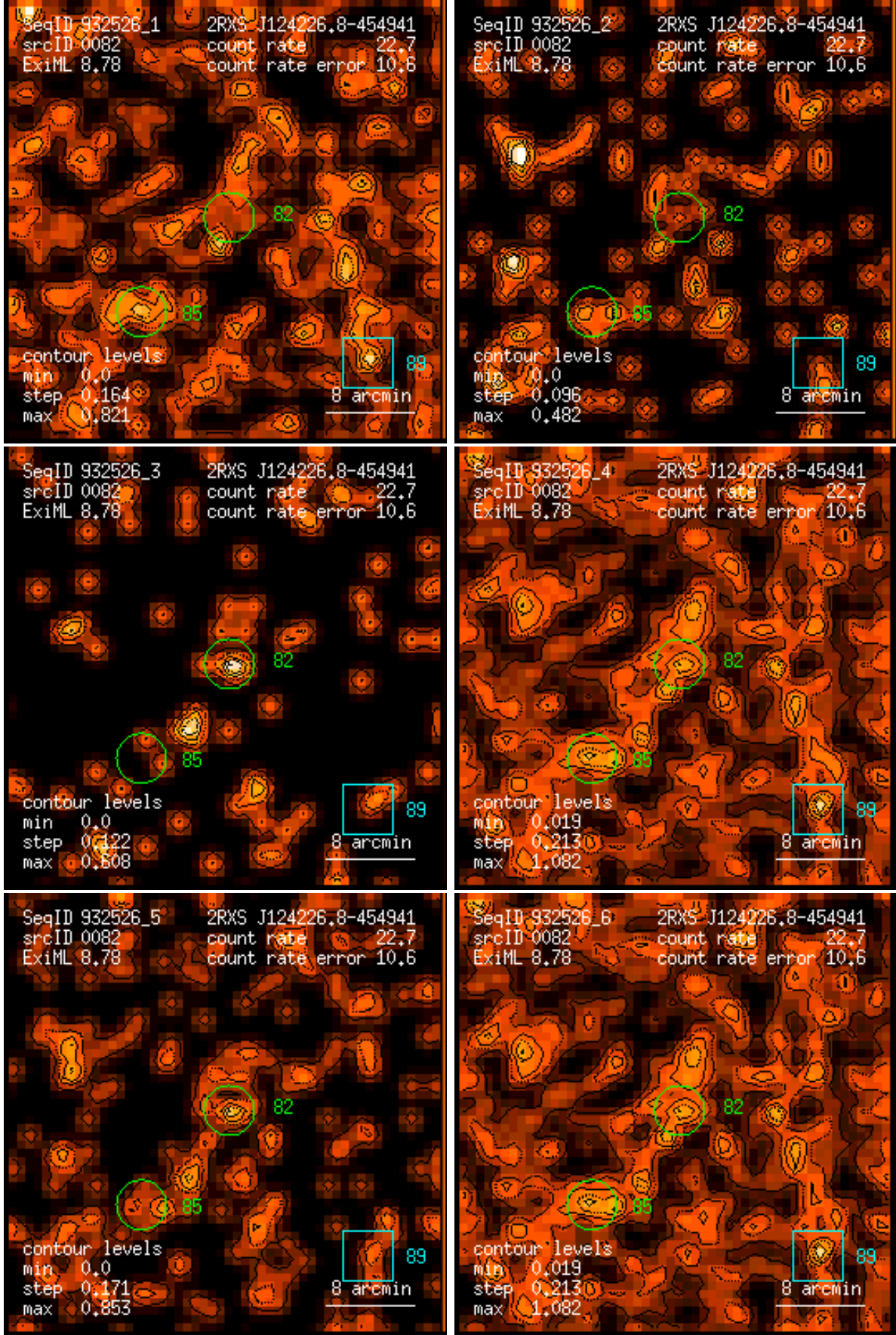
Figure 82: RASS 932526: detection 0082: band rate images, Gaussian filter: (1) PSPC channels 11 – 41, (2) 52 – 90, (3) 91 – 201, (4) 11 – 235, (5) 52 – 201, (6) 11 – 201. Broad band rates in counts/ks. Band rate contour levels in counts/ks/arcmin 2 .
