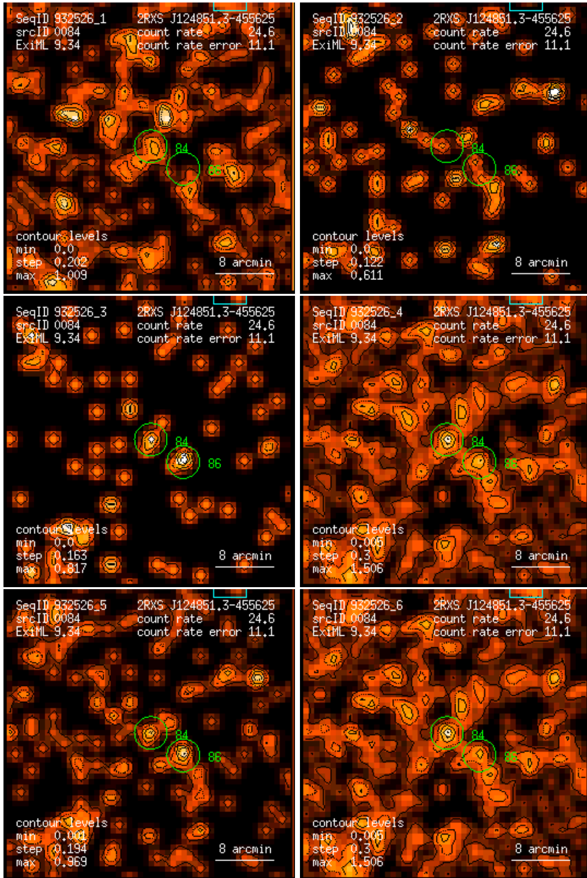
Figure 84: RASS 932526: detection 0084: band rate images, Gaussian filter: (1) PSPC channels 11 – 41, (2) 52 – 90, (3) 91 – 201, (4) 11 – 235, (5) 52 – 201, (6) 11 – 201. Broad band rates in counts/ks. Band rate contour levels in counts/ks/arcmin 2 .
