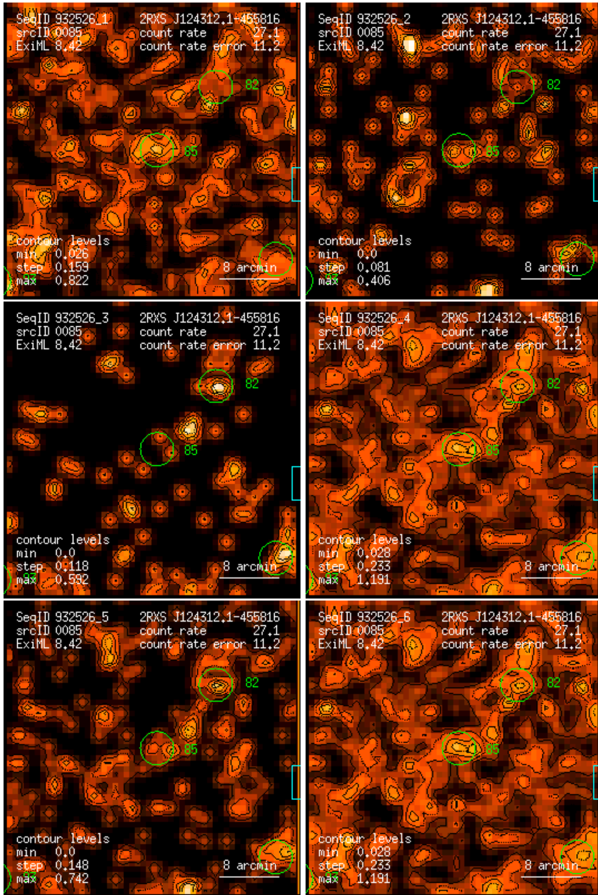
Figure 85: RASS 932526: detection 0085: band rate images, Gaussian filter: (1) PSPC channels 11 – 41, (2) 52 – 90, (3) 91 – 201, (4) 11 – 235, (5) 52 – 201, (6) 11 – 201. Broad band rates in counts/ks. Band rate contour levels in counts/ks/arcmin 2 .
