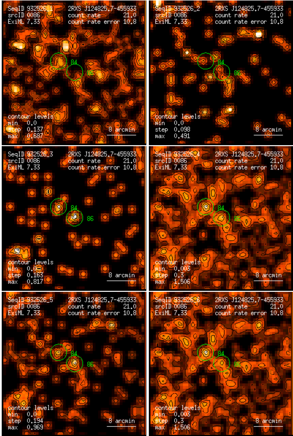
Figure 86: RASS 932526: detection 0086: band rate images, Gaussian filter: (1) PSPC channels 11 – 41, (2) 52 – 90, (3) 91 – 201, (4) 11 – 235, (5) 52 – 201, (6) 11 – 201. Broad band rates in counts/ks. Band rate contour levels in counts/ks/arcmin 2 .
