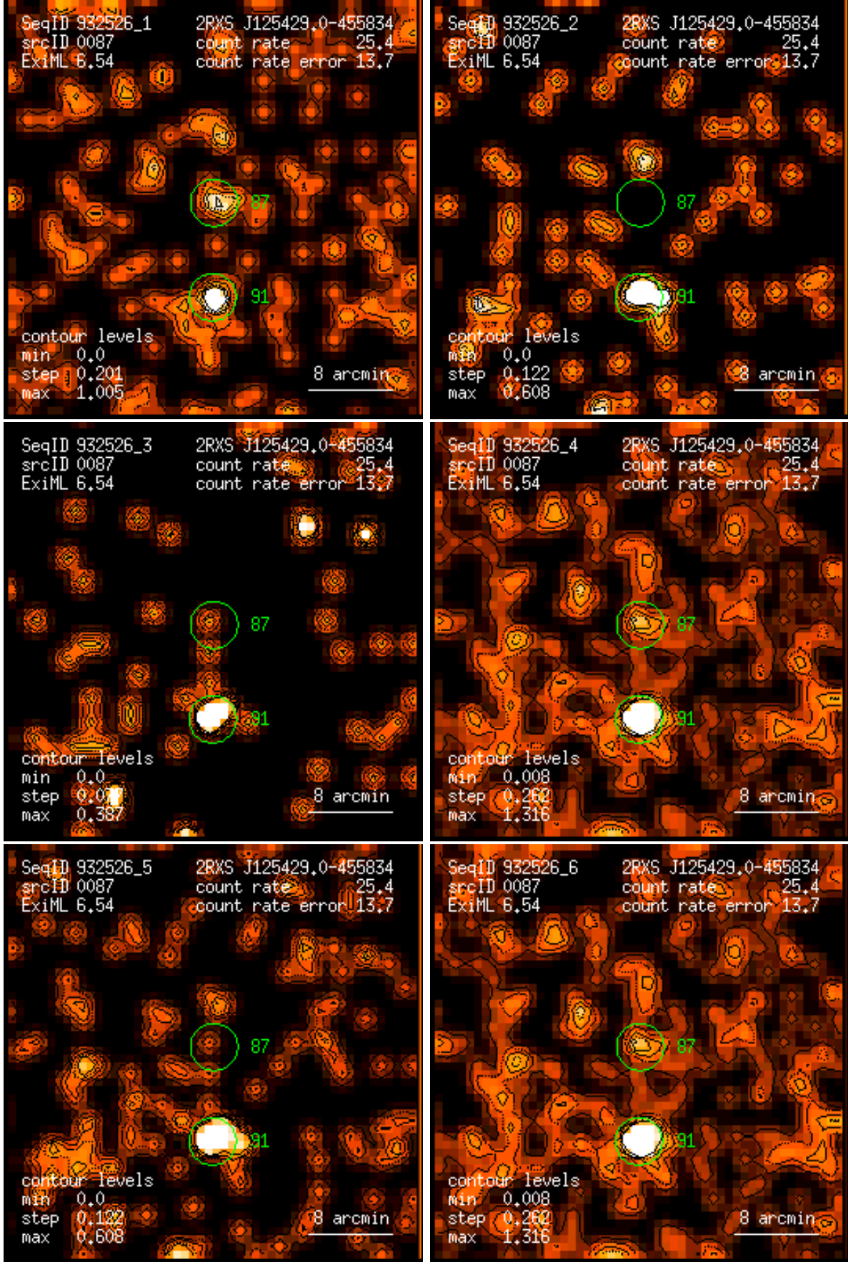
Figure 87: RASS 932526: detection 0087: band rate images, Gaussian filter: (1) PSPC channels 11 – 41, (2) 52 – 90, (3) 91 – 201, (4) 11 – 235, (5) 52 – 201, (6) 11 – 201. Broad band rates in counts/ks. Band rate contour levels in counts/ks/arcmin 2 .
