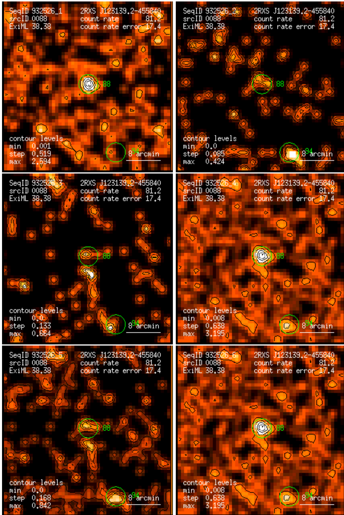
Figure 88: RASS 932526: detection 0088: band rate images, Gaussian filter: (1) PSPC channels 11 – 41, (2) 52 – 90, (3) 91 – 201, (4) 11 – 235, (5) 52 – 201, (6) 11 – 201. Broad band rates in counts/ks. Band rate contour levels in counts/ks/arcmin 2 .
