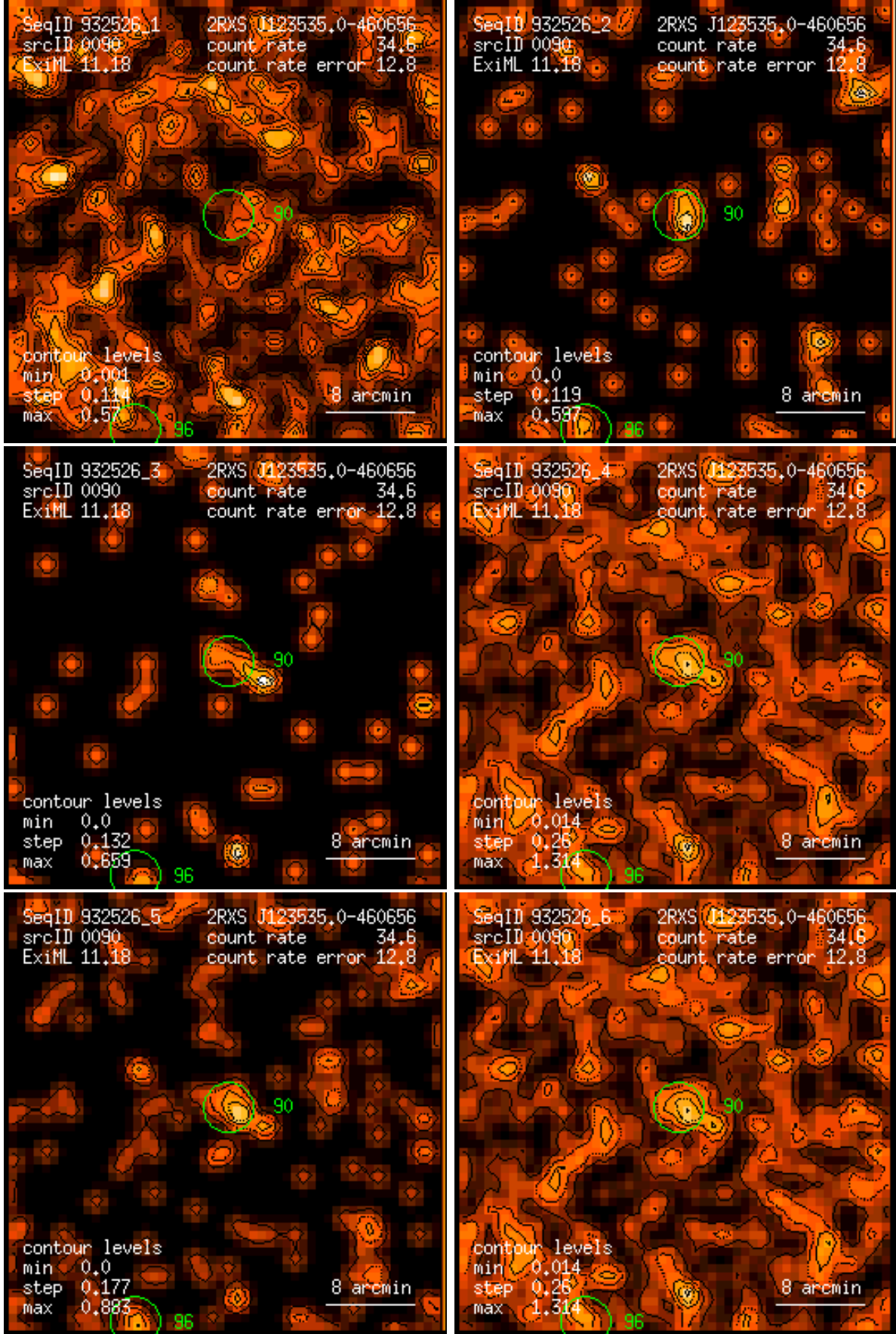
Figure 90: RASS 932526: detection 0090: band rate images, Gaussian filter: (1) PSPC channels 11 – 41, (2) 52 – 90, (3) 91 – 201, (4) 11 – 235, (5) 52 – 201, (6) 11 – 201. Broad band rates in counts/ks. Band rate contour levels in counts/ks/arcmin 2 .
