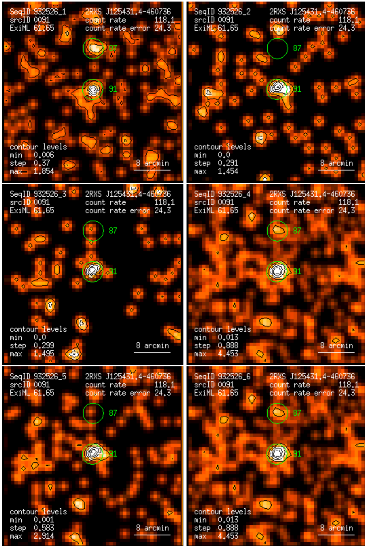
Figure 91: RASS 932526: detection 0091: band rate images, Gaussian filter: (1) PSPC channels 11 – 41, (2) 52 – 90, (3) 91 – 201, (4) 11 – 235, (5) 52 – 201, (6) 11 – 201. Broad band rates in counts/ks. Band rate contour levels in counts/ks/arcmin 2 .
