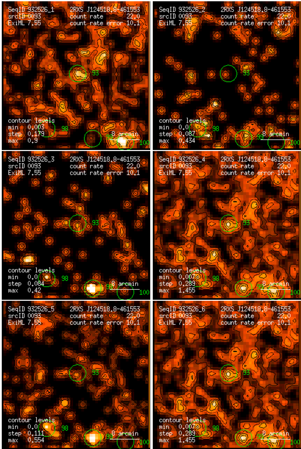
Figure 93: RASS 932526: detection 0093: band rate images, Gaussian filter: (1) PSPC channels 11 – 41, (2) 52 – 90, (3) 91 – 201, (4) 11 – 235, (5) 52 – 201, (6) 11 – 201. Broad band rates in counts/ks. Band rate contour levels in counts/ks/arcmin 2 .
