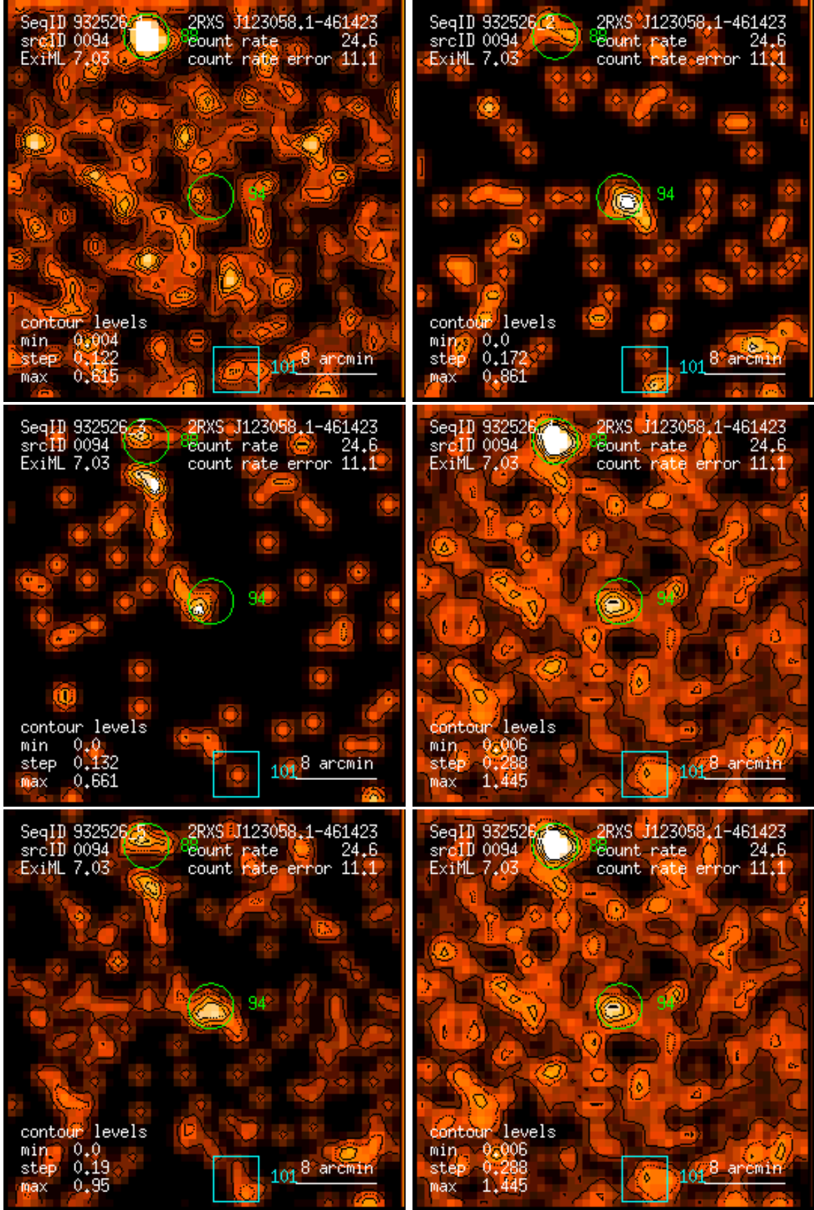
Figure 94: RASS 932526: detection 0094: band rate images, Gaussian filter: (1) PSPC channels 11 – 41, (2) 52 – 90, (3) 91 – 201, (4) 11 – 235, (5) 52 – 201, (6) 11 – 201. Broad band rates in counts/ks. Band rate contour levels in counts/ks/arcmin 2 .
