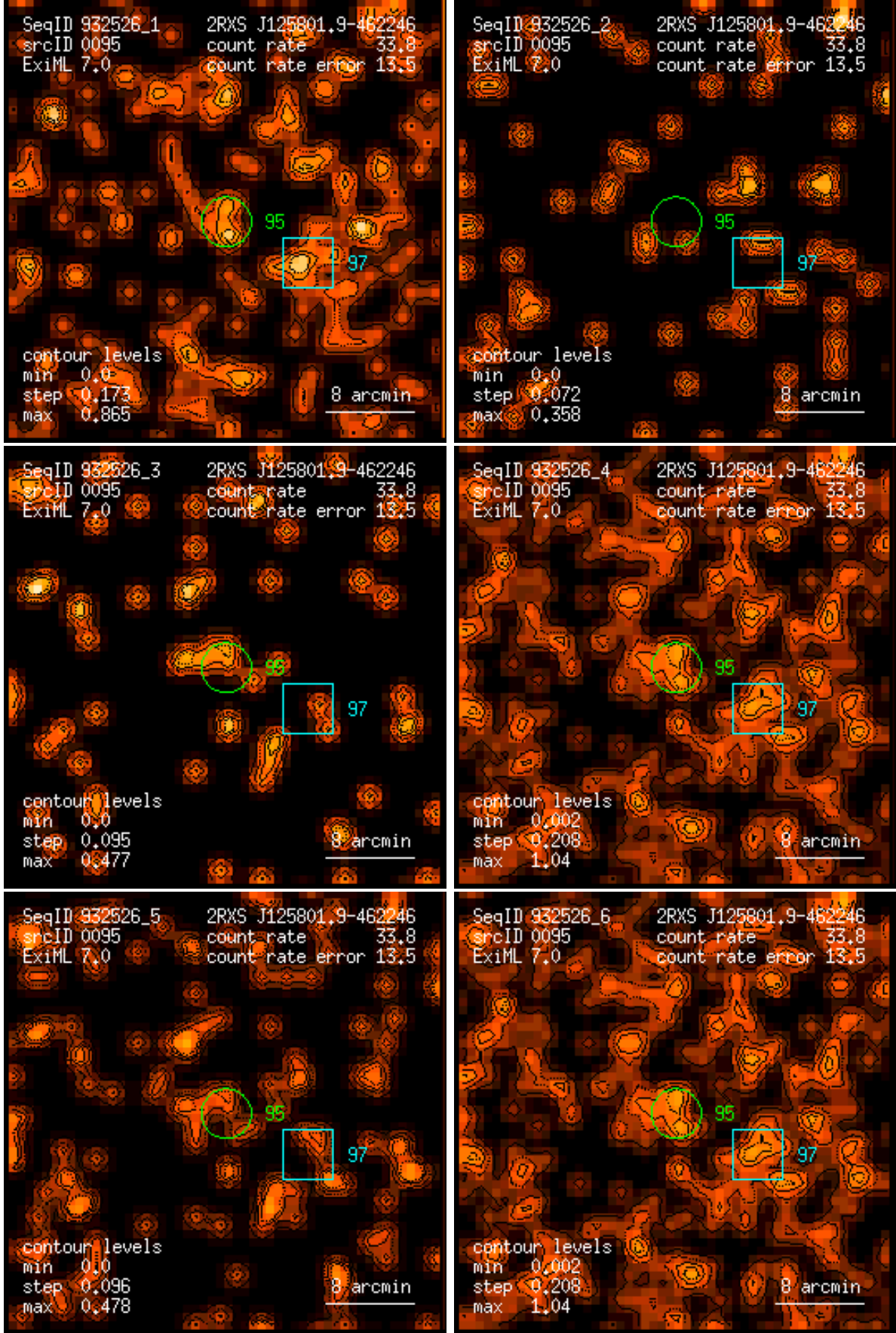
Figure 95: RASS 932526: detection 0095: band rate images, Gaussian filter: (1) PSPC channels 11 – 41, (2) 52 – 90, (3) 91 – 201, (4) 11 – 235, (5) 52 – 201, (6) 11 – 201. Broad band rates in counts/ks. Band rate contour levels in counts/ks/arcmin 2 .
