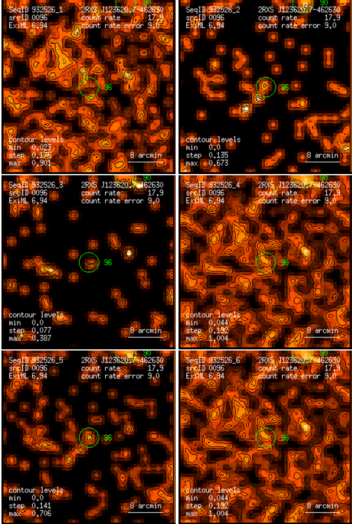
Figure 96: RASS 932526: detection 0096: band rate images, Gaussian filter: (1) PSPC channels 11 – 41, (2) 52 – 90, (3) 91 – 201, (4) 11 – 235, (5) 52 – 201, (6) 11 – 201. Broad band rates in counts/ks. Band rate contour levels in counts/ks/arcmin 2 .
