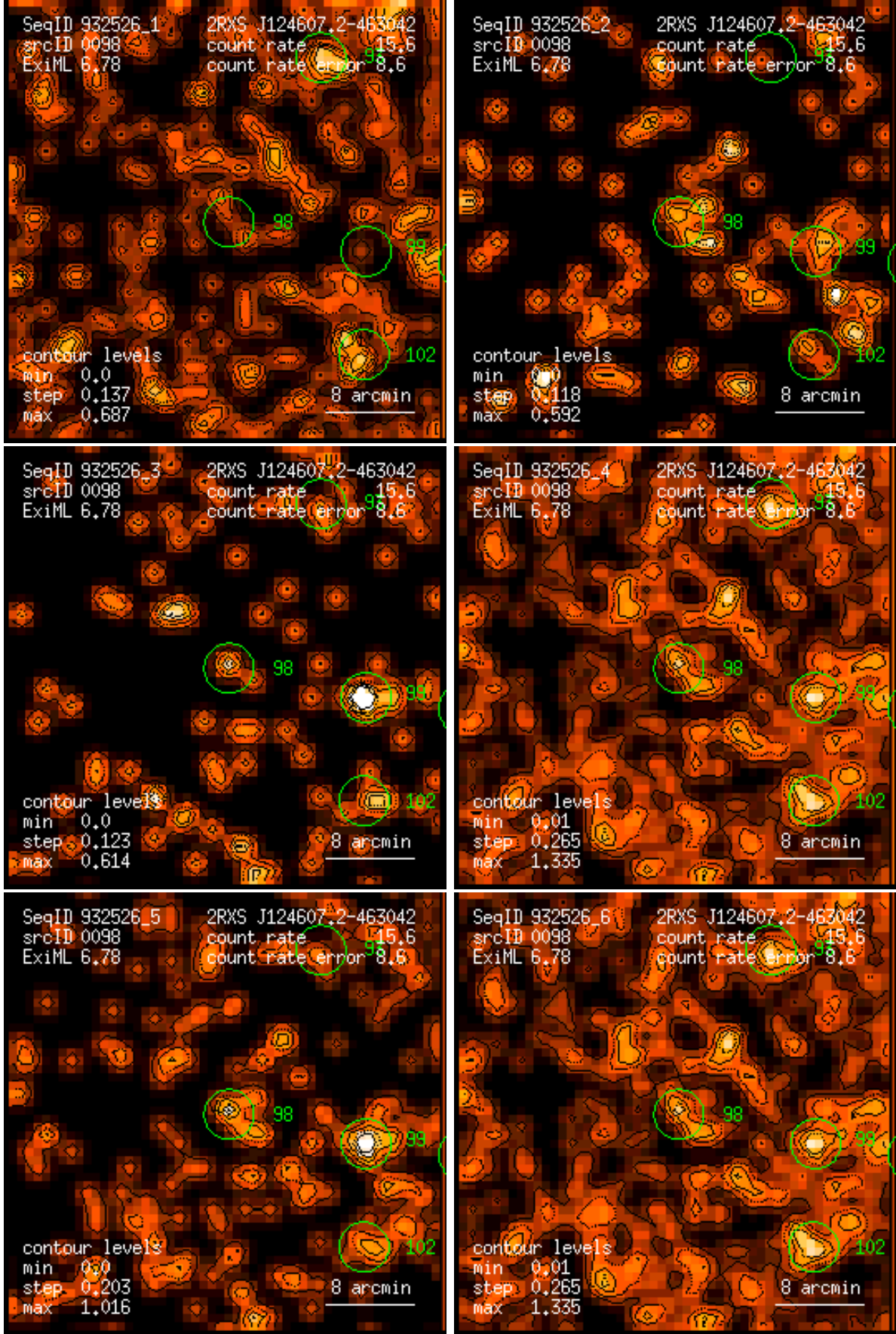
Figure 98: RASS 932526: detection 0098: band rate images, Gaussian filter: (1) PSPC channels 11 – 41, (2) 52 – 90, (3) 91 – 201, (4) 11 – 235, (5) 52 – 201, (6) 11 – 201. Broad band rates in counts/ks. Band rate contour levels in counts/ks/arcmin 2 .
