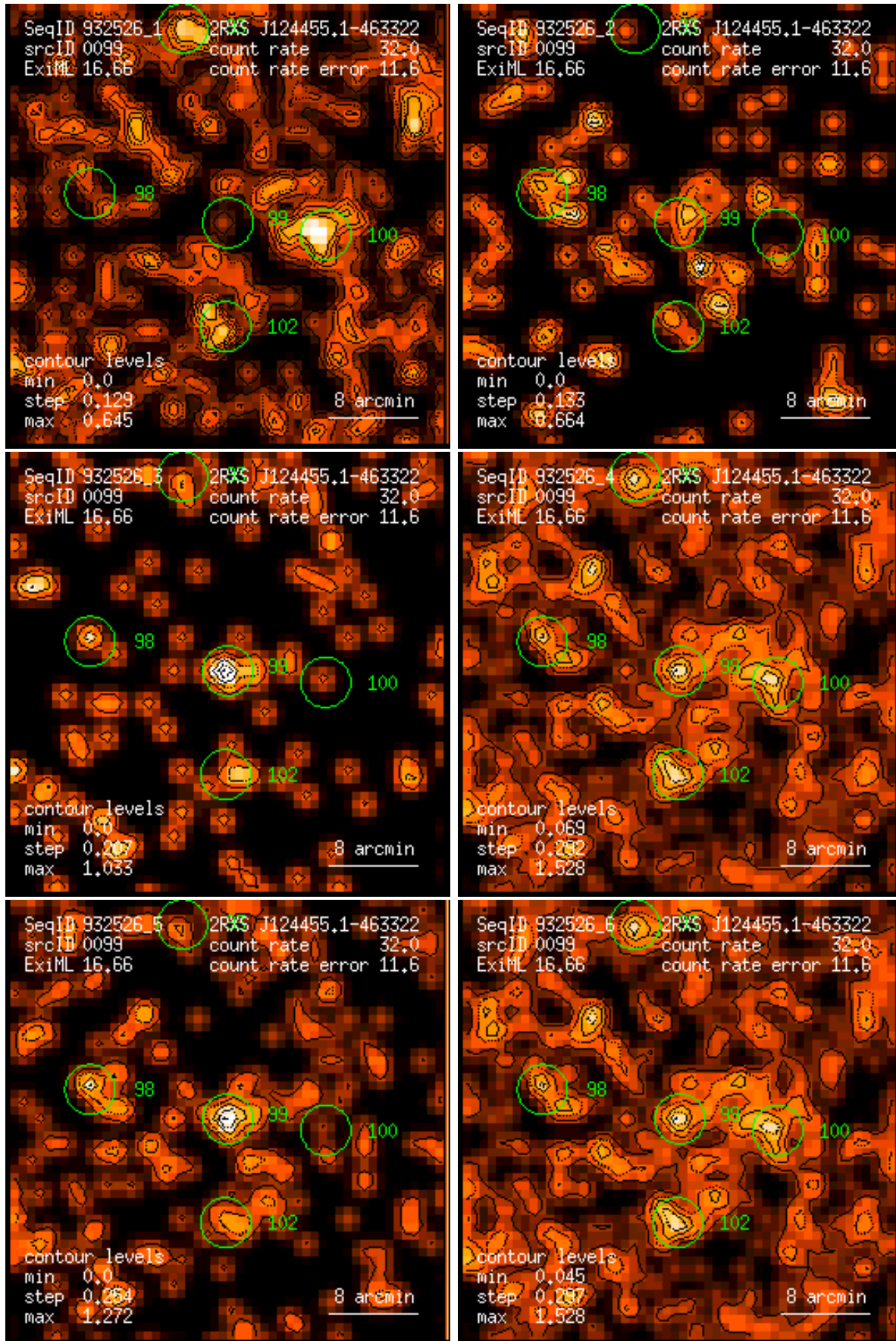
Figure 99: RASS 932526: detection 0099: band rate images, Gaussian filter: (1) PSPC channels 11 – 41, (2) 52 – 90, (3) 91 – 201, (4) 11 – 235, (5) 52 – 201, (6) 11 – 201. Broad band rates in counts/ks. Band rate contour levels in counts/ks/arcmin 2 .
