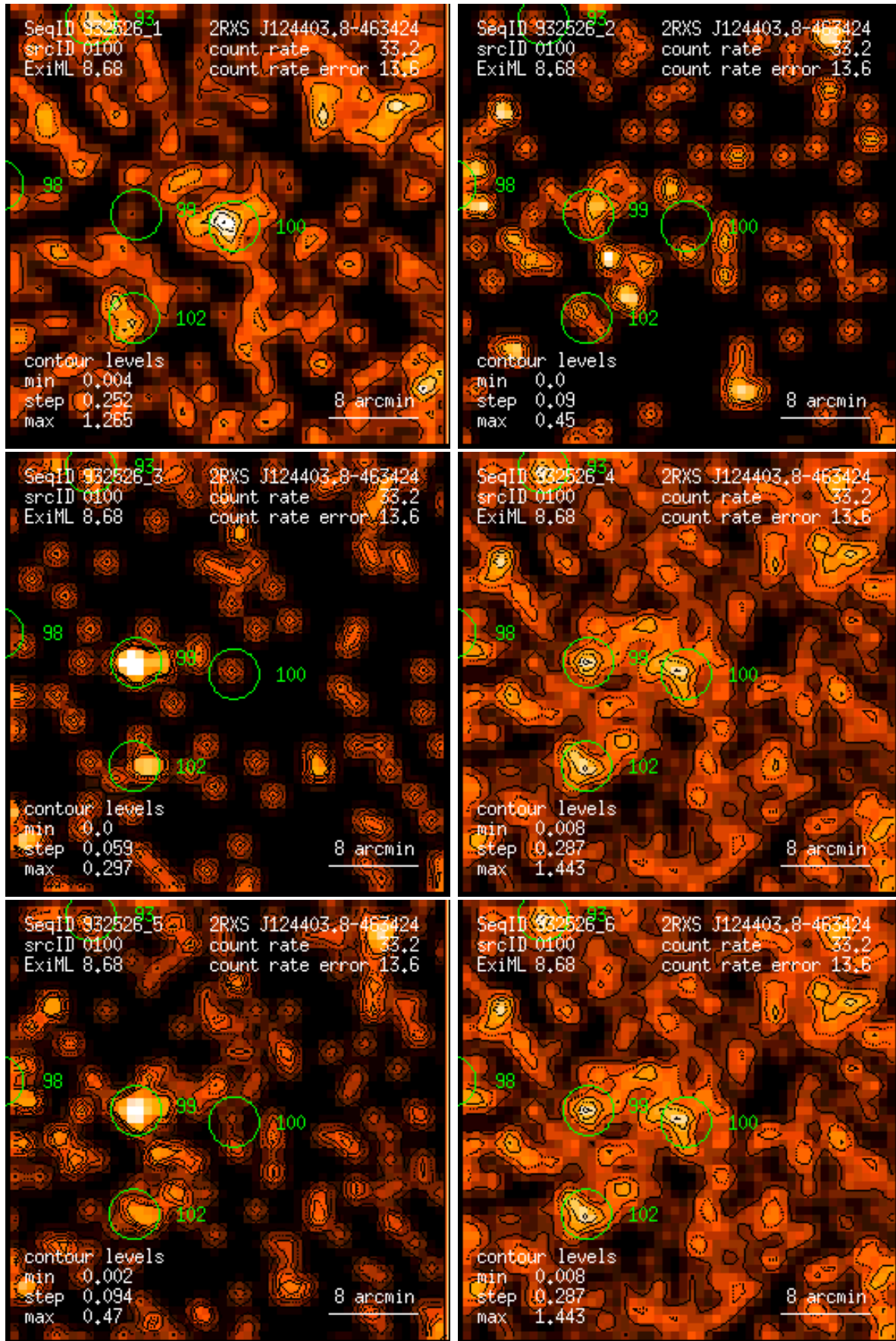
Figure 100: RASS 932526: detection 0100: band rate images, Gaussian filter: (1) PSPC channels 11 – 41, (2) 52 – 90, (3) 91 – 201, (4) 11 – 235, (5) 52 – 201, (6) 11 – 201. Broad band rates in counts/ks. Band rate contour levels in counts/ks/arcmin 2 .
