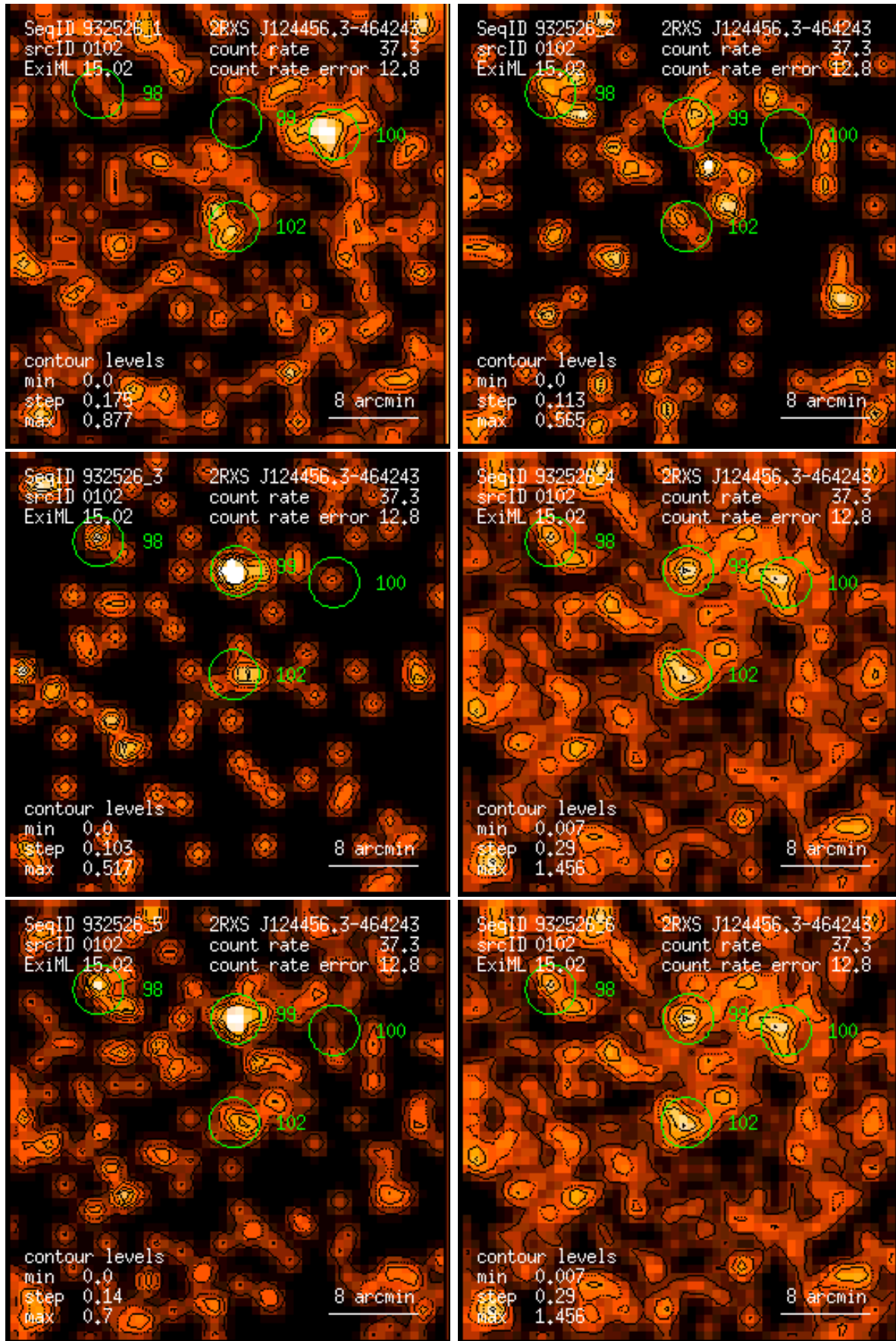
Figure 102: RASS 932526: detection 0102: band rate images, Gaussian filter: (1) PSPC channels 11 – 41, (2) 52 – 90, (3) 91 – 201, (4) 11 – 235, (5) 52 – 201, (6) 11 – 201. Broad band rates in counts/ks. Band rate contour levels in counts/ks/arcmin 2 .
