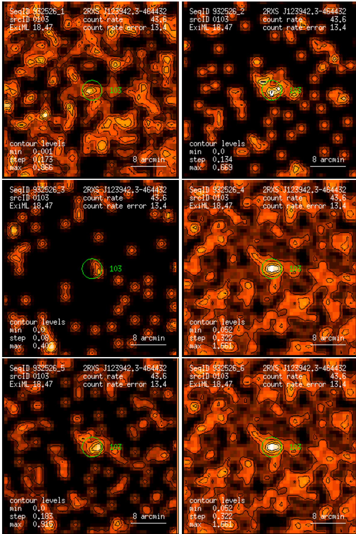
Figure 103: RASS 932526: detection 0103: band rate images, Gaussian filter: (1) PSPC channels 11 – 41, (2) 52 – 90, (3) 91 – 201, (4) 11 – 235, (5) 52 – 201, (6) 11 – 201. Broad band rates in counts/ks. Band rate contour levels in counts/ks/arcmin 2 .
