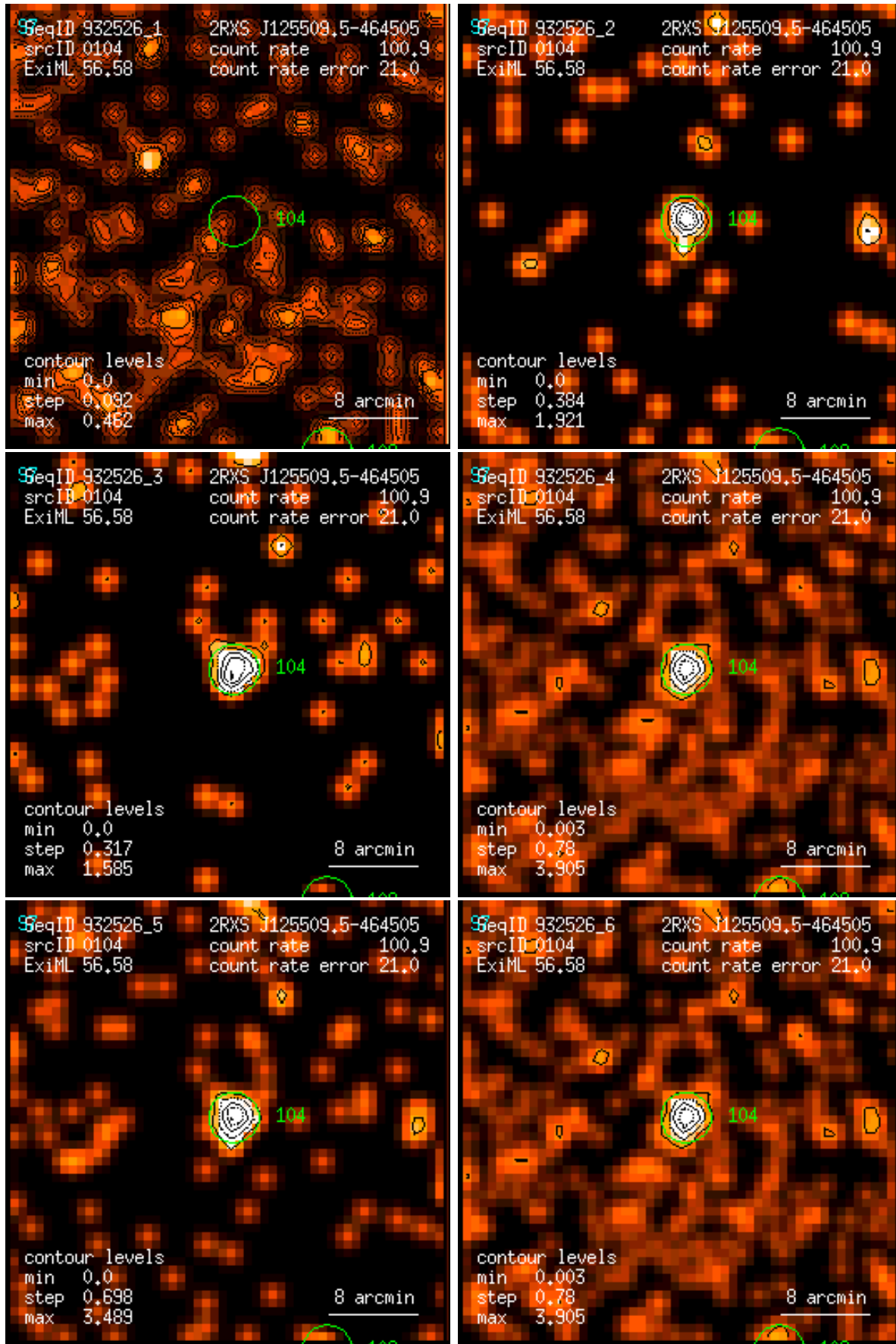
Figure 104: RASS 932526: detection 0104: band rate images, Gaussian filter: (1) PSPC channels 11 – 41, (2) 52 – 90, (3) 91 – 201, (4) 11 – 235, (5) 52 – 201, (6) 11 – 201. Broad band rates in counts/ks. Band rate contour levels in counts/ks/arcmin 2 .
