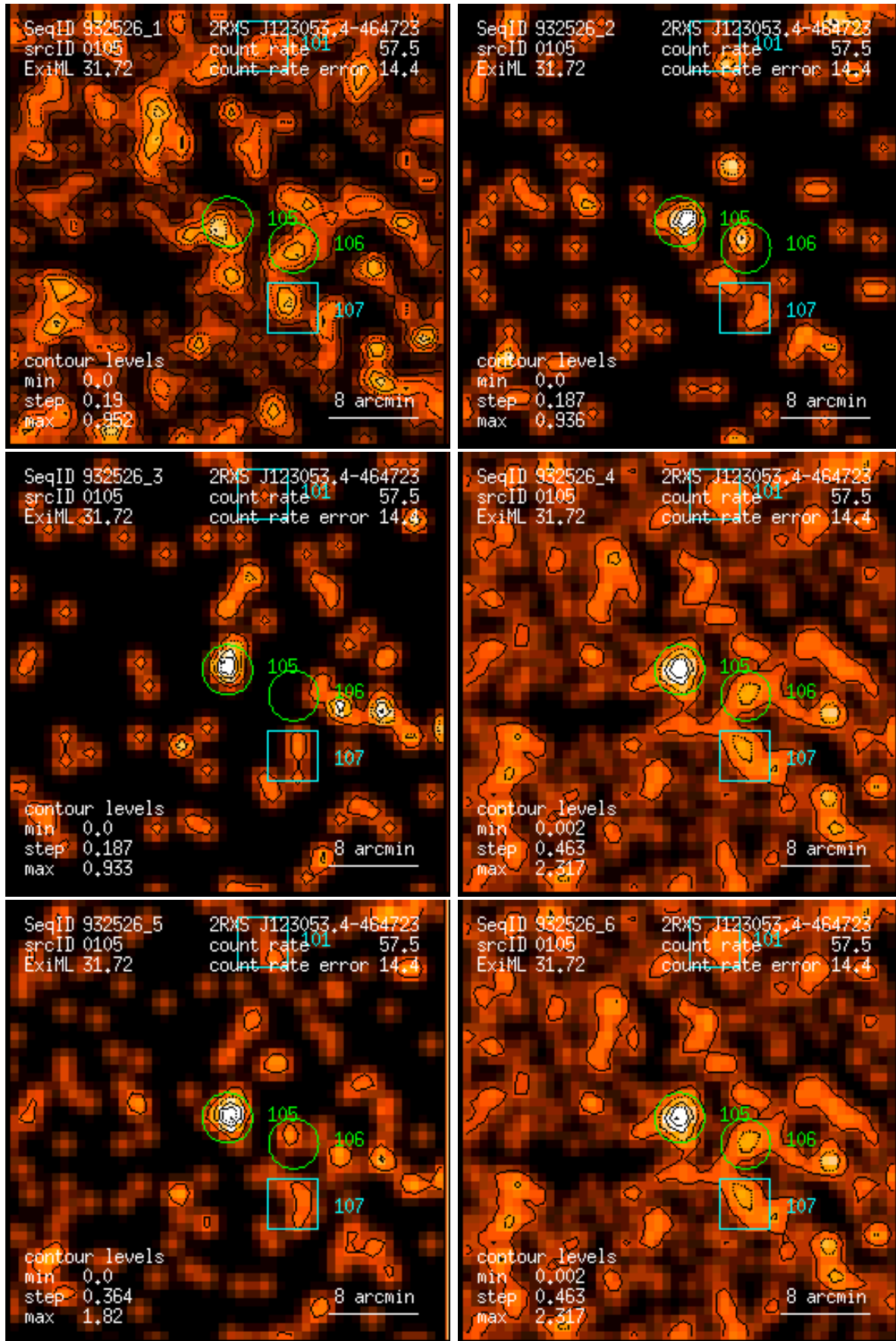
Figure 105: RASS 932526: detection 0105: band rate images, Gaussian filter: (1) PSPC channels 11 – 41, (2) 52 – 90, (3) 91 – 201, (4) 11 – 235, (5) 52 – 201, (6) 11 – 201. Broad band rates in counts/ks. Band rate contour levels in counts/ks/arcmin 2 .
