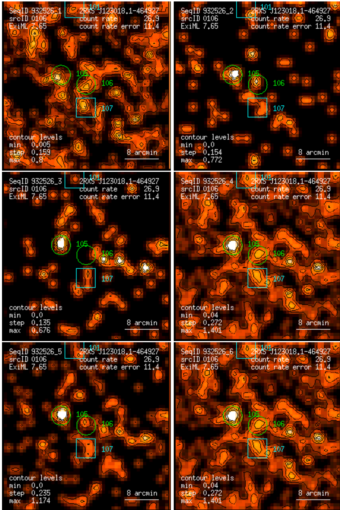
Figure 106: RASS 932526: detection 0106: band rate images, Gaussian filter: (1) PSPC channels 11 – 41, (2) 52 – 90, (3) 91 – 201, (4) 11 – 235, (5) 52 – 201, (6) 11 – 201. Broad band rates in counts/ks. Band rate contour levels in counts/ks/arcmin 2 .
