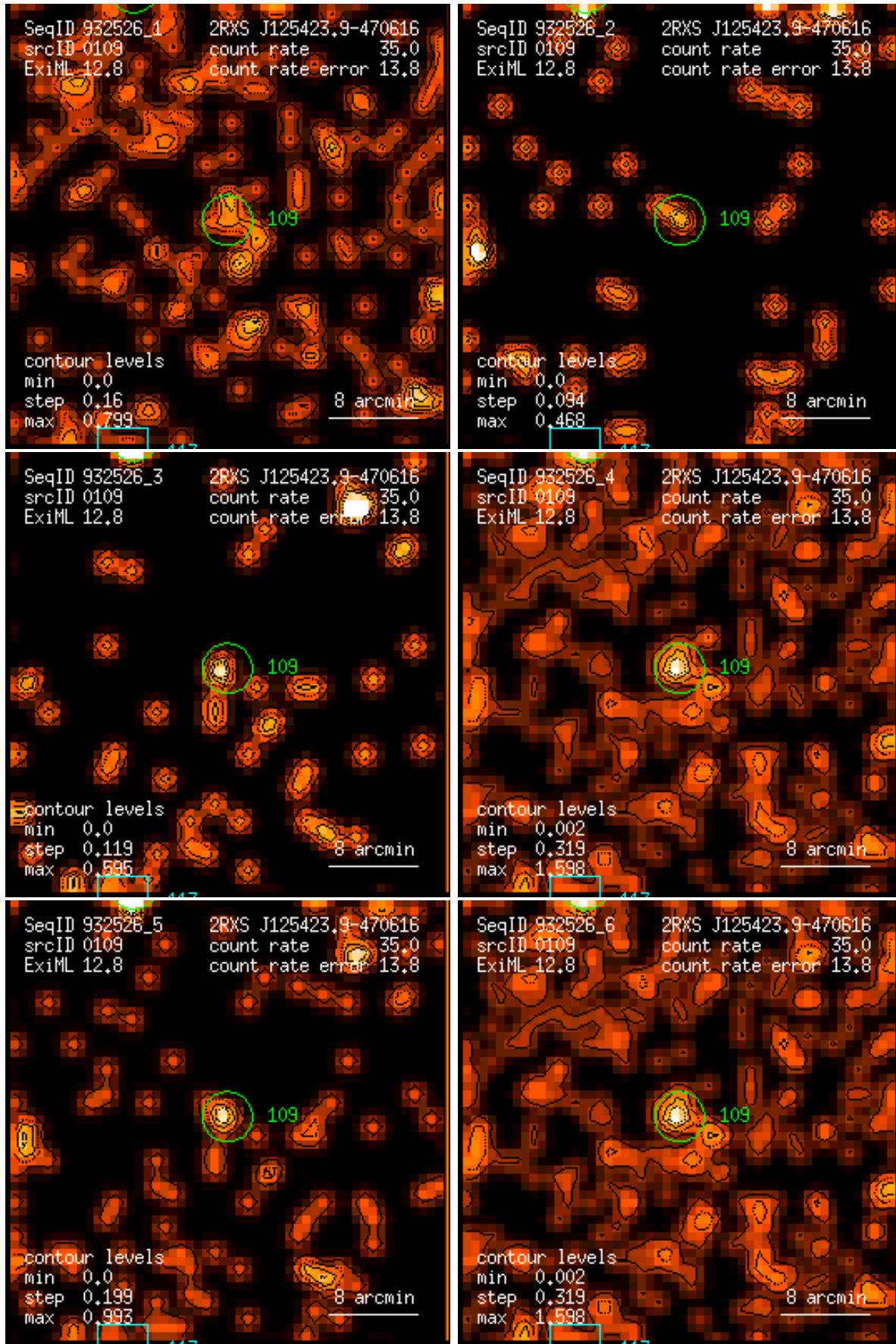
Figure 109: RASS 932526: detection 0109: band rate images, Gaussian filter: (1) PSPC channels 11 – 41, (2) 52 – 90, (3) 91 – 201, (4) 11 – 235, (5) 52 – 201, (6) 11 – 201. Broad band rates in counts/ks. Band rate contour levels in counts/ks/arcmin 2 .
