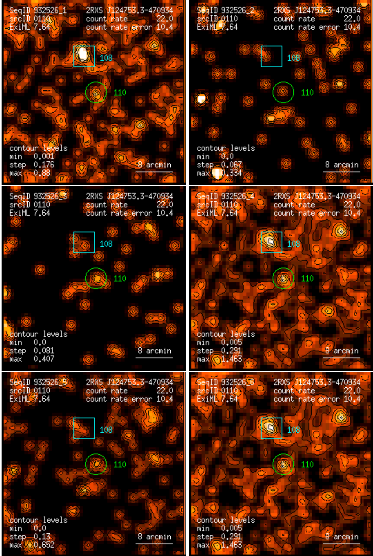
Figure 110: RASS 932526: detection 0110: band rate images, Gaussian filter: (1) PSPC channels 11 – 41, (2) 52 – 90, (3) 91 – 201, (4) 11 – 235, (5) 52 – 201, (6) 11 – 201. Broad band rates in counts/ks. Band rate contour levels in counts/ks/arcmin 2 .
