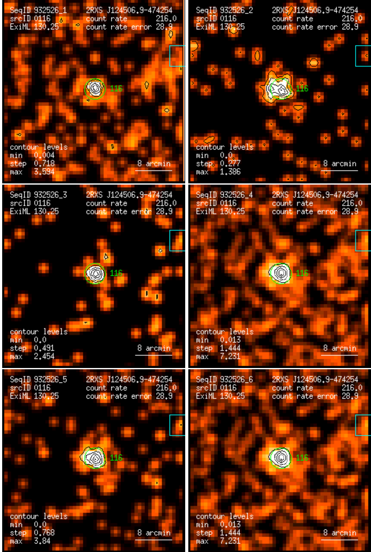
Figure 116: RASS 932526: detection 0116: band rate images, Gaussian filter: (1) PSPC channels 11 – 41, (2) 52 – 90, (3) 91 – 201, (4) 11 – 235, (5) 52 – 201, (6) 11 – 201. Broad band rates in counts/ks. Band rate contour levels in counts/ks/arcmin 2 .
