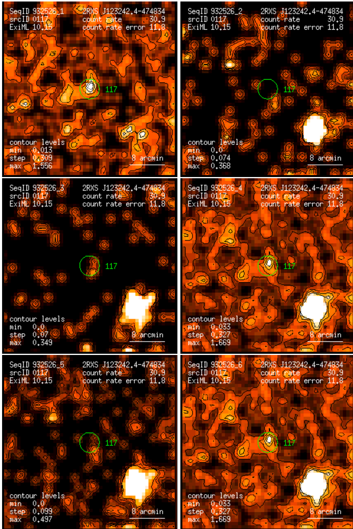
Figure 117: RASS 932526: detection 0117: band rate images, Gaussian filter: (1) PSPC channels 11 – 41, (2) 52 – 90, (3) 91 – 201, (4) 11 – 235, (5) 52 – 201, (6) 11 – 201. Broad band rates in counts/ks. Band rate contour levels in counts/ks/arcmin 2 .
