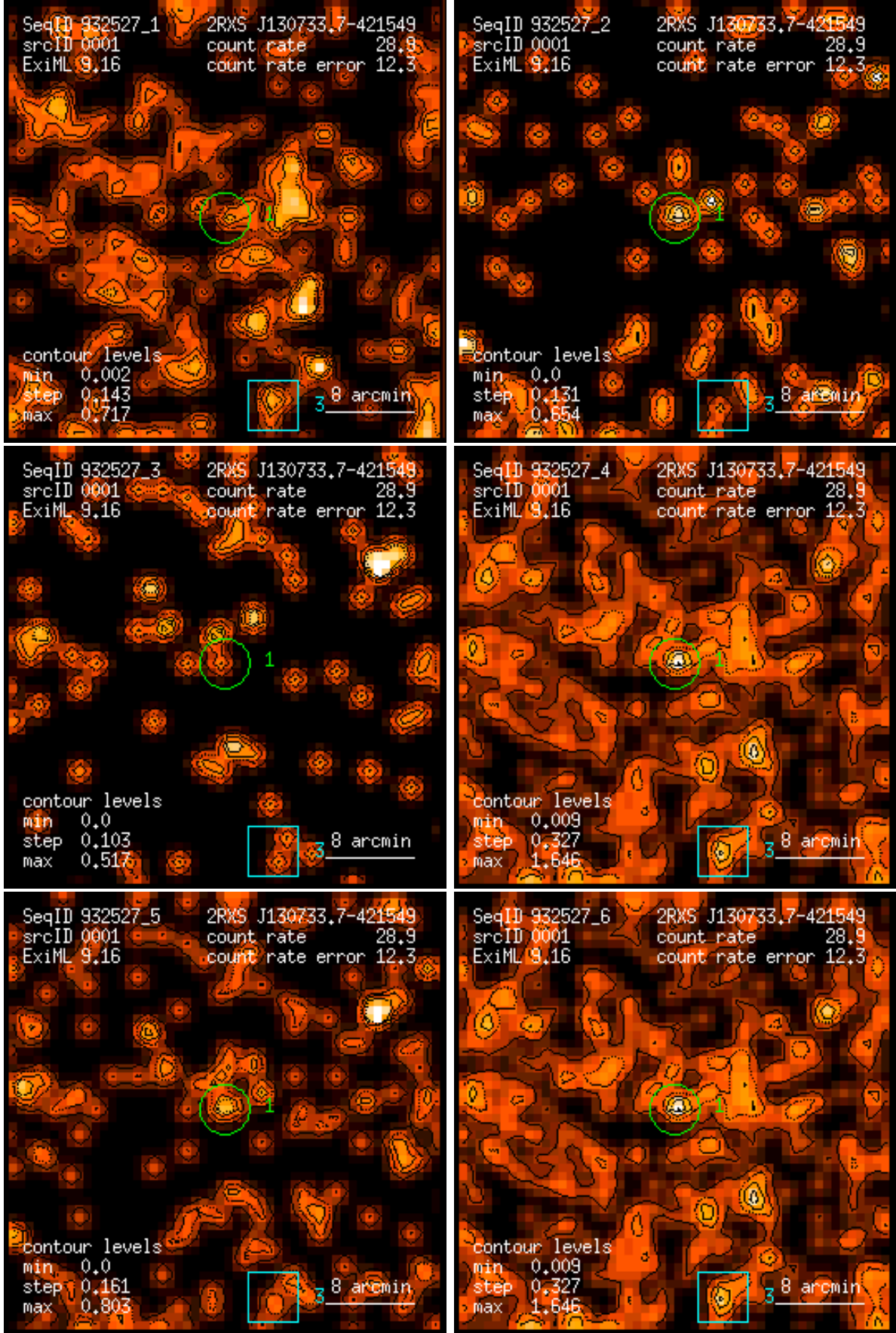
Figure 1: RASS 932527: detection 0001: band rate images, Gaussian filter: (1) PSPC channels 11 – 41, (2) 52 – 90, (3) 91 – 201, (4) 11 – 235, (5) 52 – 201, (6) 11 – 201. Broad band rates in counts/ks. Band rate contour levels in counts/ks/arcmin 2 .
