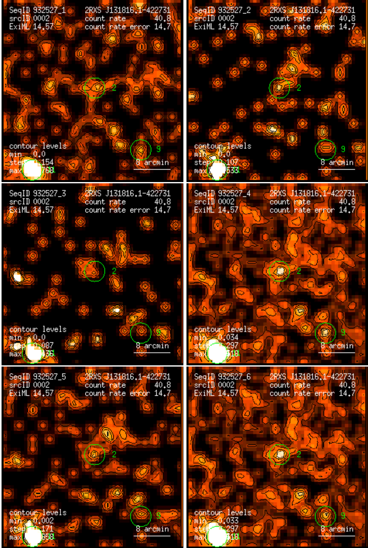
Figure 2: RASS 932527: detection 0002: band rate images, Gaussian filter: (1) PSPC channels 11 – 41, (2) 52 – 90, (3) 91 – 201, (4) 11 – 235, (5) 52 – 201, (6) 11 – 201. Broad band rates in counts/ks. Band rate contour levels in counts/ks/arcmin 2 .
