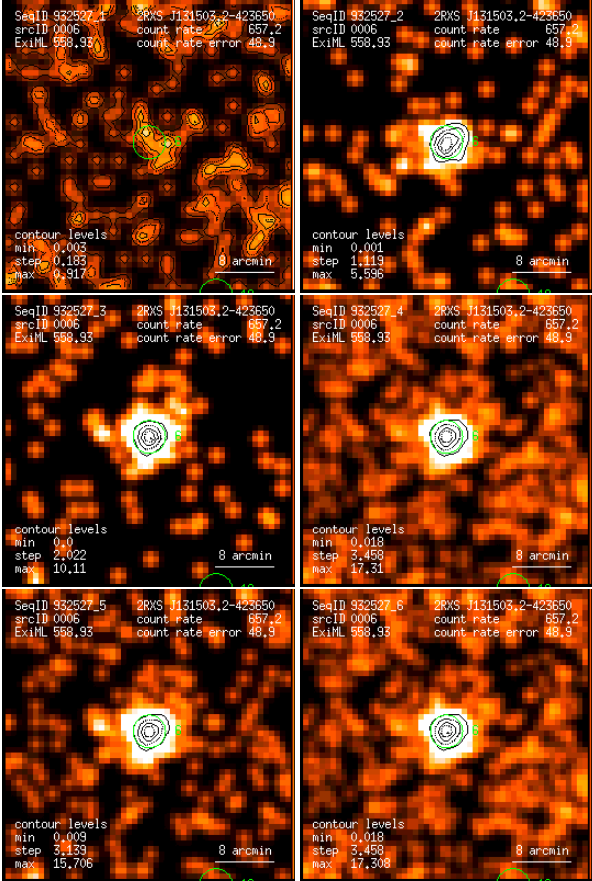
Figure 6: RASS 932527: detection 0006: band rate images, Gaussian filter: (1) PSPC channels 11 – 41, (2) 52 – 90, (3) 91 – 201, (4) 11 – 235, (5) 52 – 201, (6) 11 – 201. Broad band rates in counts/ks. Band rate contour levels in counts/ks/arcmin 2 .
