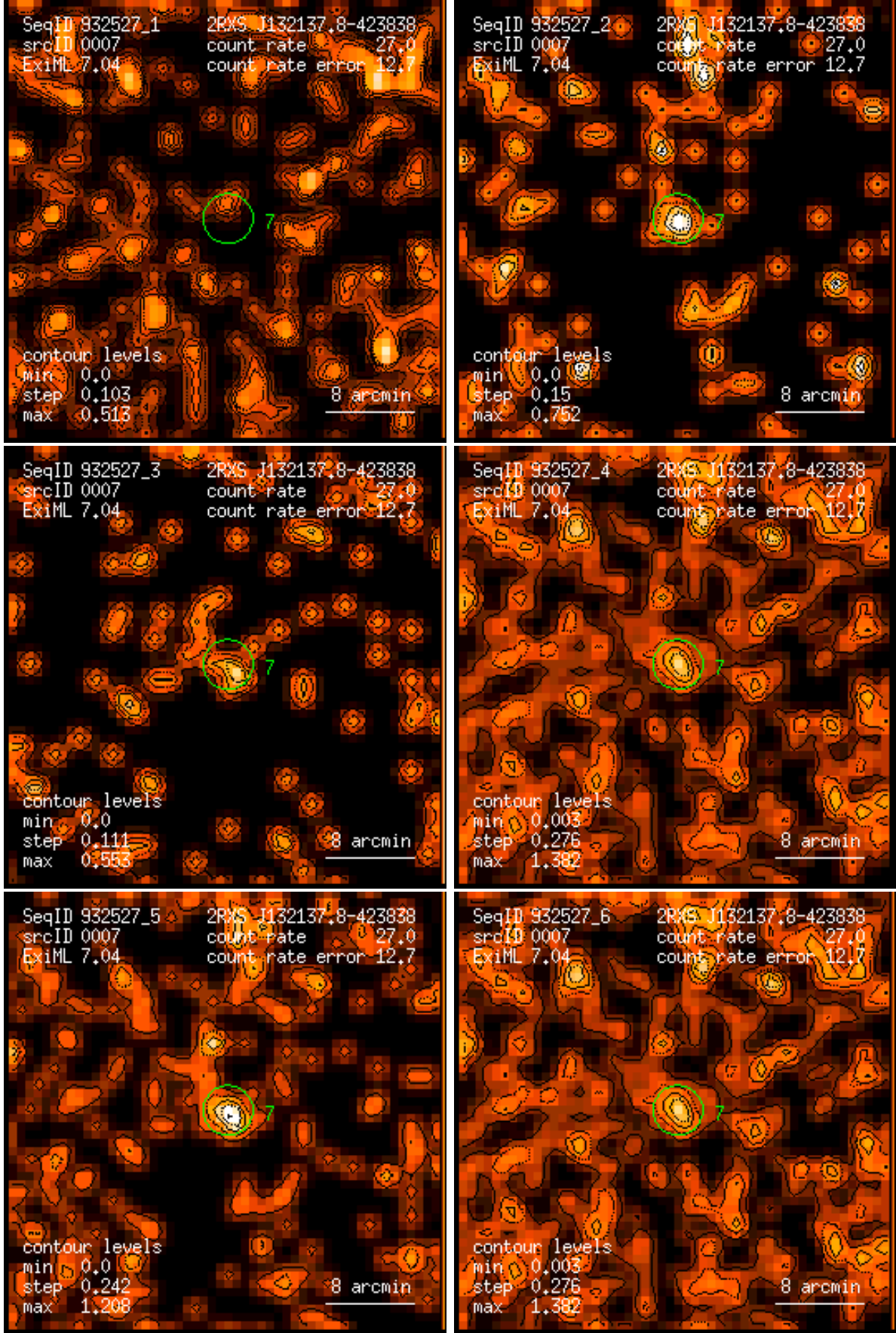
Figure 7: RASS 932527: detection 0007: band rate images, Gaussian filter: (1) PSPC channels 11 – 41, (2) 52 – 90, (3) 91 – 201, (4) 11 – 235, (5) 52 – 201, (6) 11 – 201. Broad band rates in counts/ks. Band rate contour levels in counts/ks/arcmin 2 .
