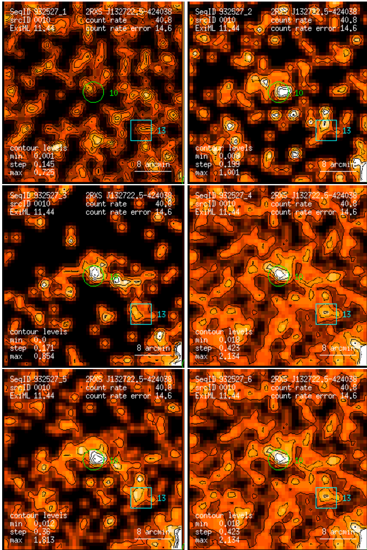
Figure 10: RASS 932527: detection 0010: band rate images, Gaussian filter: (1) PSPC channels 11 – 41, (2) 52 – 90, (3) 91 – 201, (4) 11 – 235, (5) 52 – 201, (6) 11 – 201. Broad band rates in counts/ks. Band rate contour levels in counts/ks/arcmin 2 .
