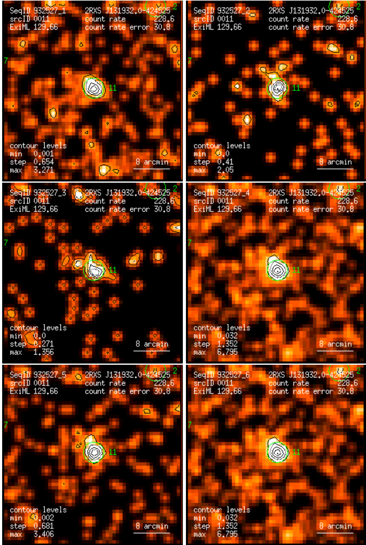
Figure 11: RASS 932527: detection 0011: band rate images, Gaussian filter: (1) PSPC channels 11 – 41, (2) 52 – 90, (3) 91 – 201, (4) 11 – 235, (5) 52 – 201, (6) 11 – 201. Broad band rates in counts/ks. Band rate contour levels in counts/ks/arcmin 2 .
