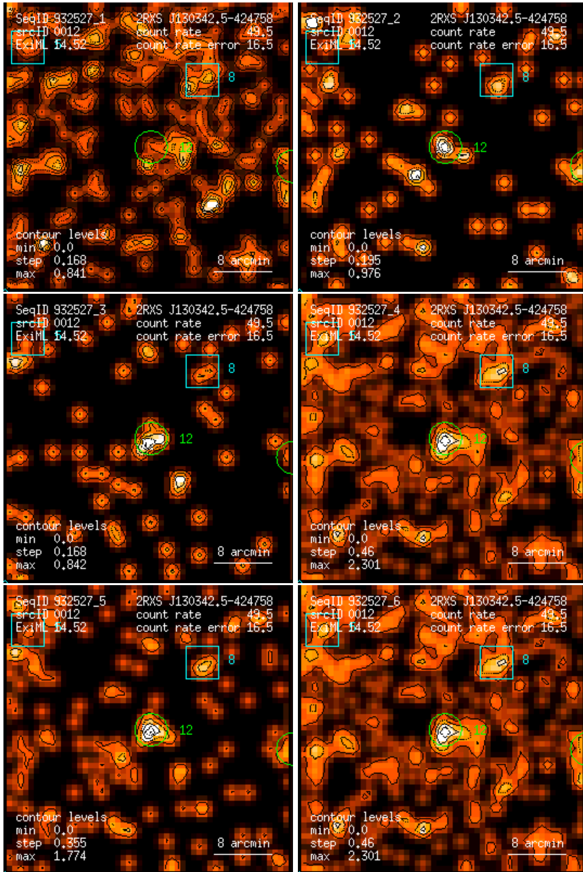
Figure 12: RASS 932527: detection 0012: band rate images, Gaussian filter: (1) PSPC channels 11 – 41, (2) 52 – 90, (3) 91 – 201, (4) 11 – 235, (5) 52 – 201, (6) 11 – 201. Broad band rates in counts/ks. Band rate contour levels in counts/ks/arcmin 2 .
