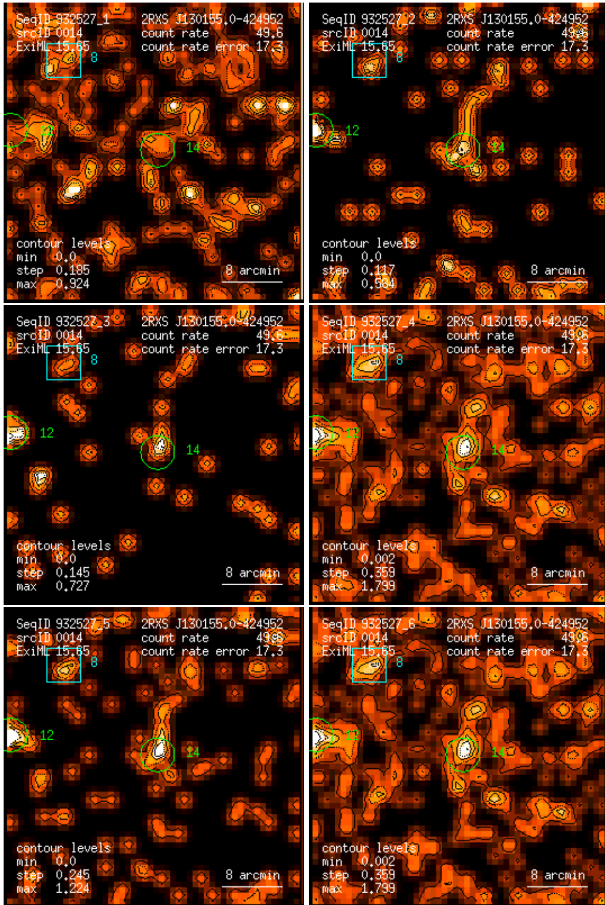
Figure 14: RASS 932527: detection 0014: band rate images, Gaussian filter: (1) PSPC channels 11 – 41, (2) 52 – 90, (3) 91 – 201, (4) 11 – 235, (5) 52 – 201, (6) 11 – 201. Broad band rates in counts/ks. Band rate contour levels in counts/ks/arcmin 2 .
