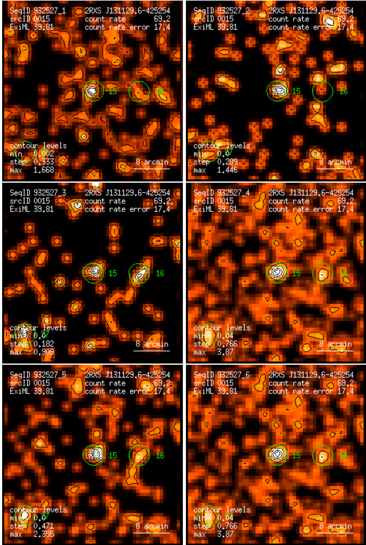
Figure 15: RASS 932527: detection 0015: band rate images, Gaussian filter: (1) PSPC channels 11 – 41, (2) 52 – 90, (3) 91 – 201, (4) 11 – 235, (5) 52 – 201, (6) 11 – 201. Broad band rates in counts/ks. Band rate contour levels in counts/ks/arcmin 2 .
