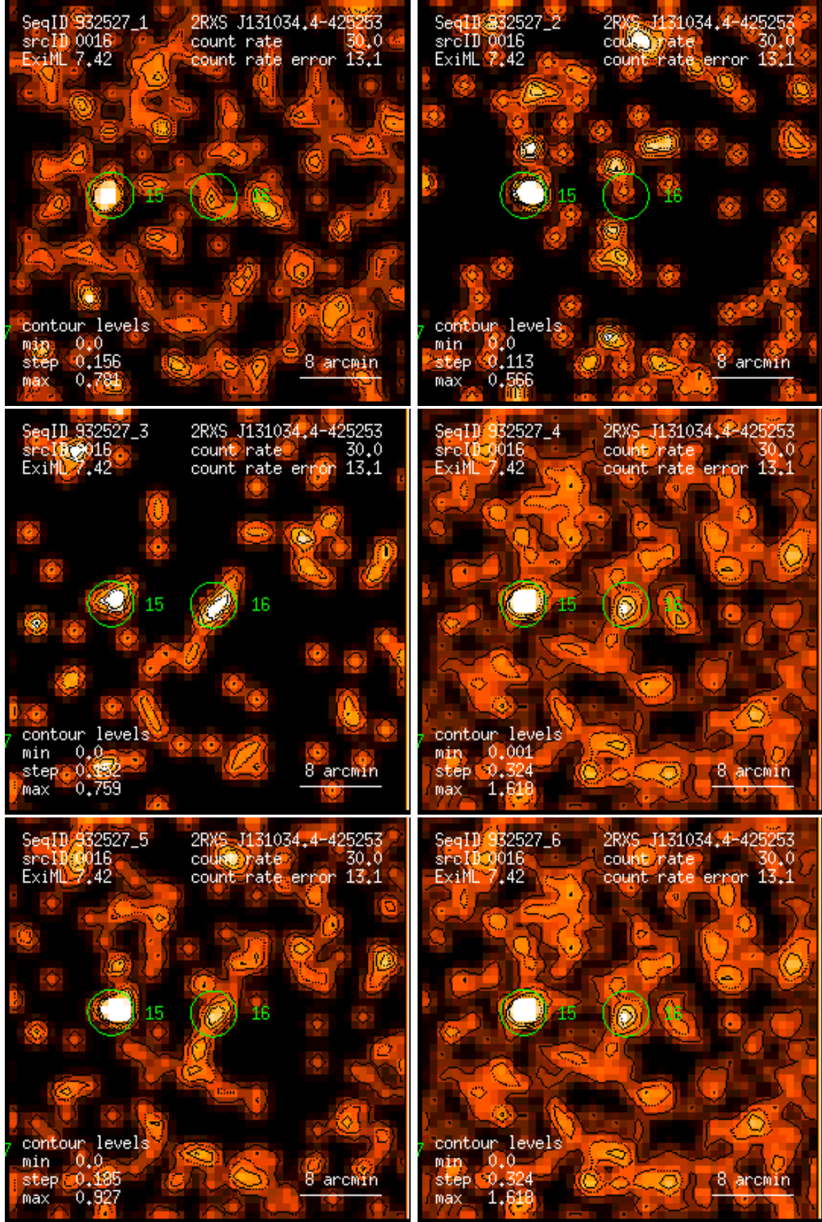
Figure 16: RASS 932527: detection 0016: band rate images, Gaussian filter: (1) PSPC channels 11 – 41, (2) 52 – 90, (3) 91 – 201, (4) 11 – 235, (5) 52 – 201, (6) 11 – 201. Broad band rates in counts/ks. Band rate contour levels in counts/ks/arcmin 2 .
