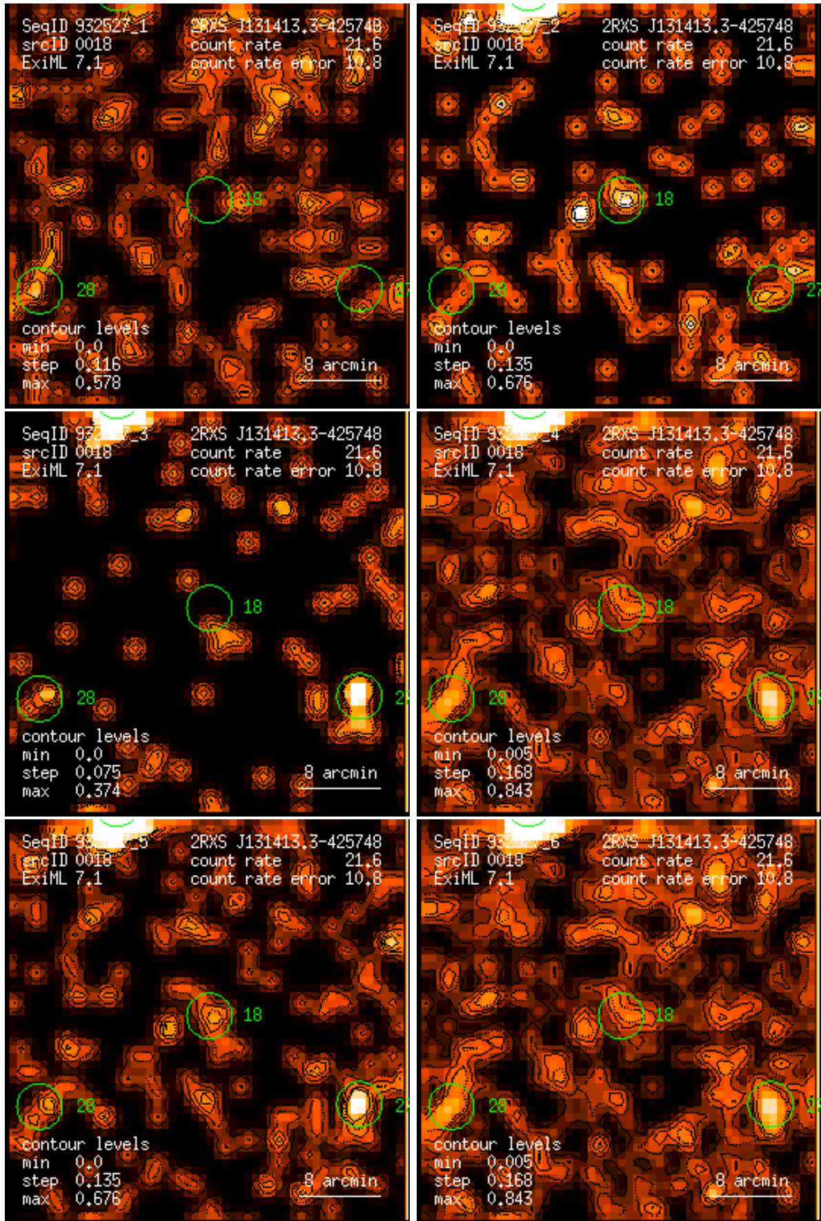
Figure 18: RASS 932527: detection 0018: band rate images, Gaussian filter: (1) PSPC channels 11 – 41, (2) 52 – 90, (3) 91 – 201, (4) 11 – 235, (5) 52 – 201, (6) 11 – 201. Broad band rates in counts/ks. Band rate contour levels in counts/ks/arcmin 2 .
