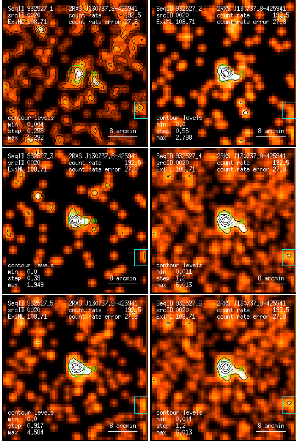
Figure 20: RASS 932527: detection 0020: band rate images, Gaussian filter: (1) PSPC channels 11 – 41, (2) 52 – 90, (3) 91 – 201, (4) 11 – 235, (5) 52 – 201, (6) 11 – 201. Broad band rates in counts/ks. Band rate contour levels in counts/ks/arcmin 2 .
