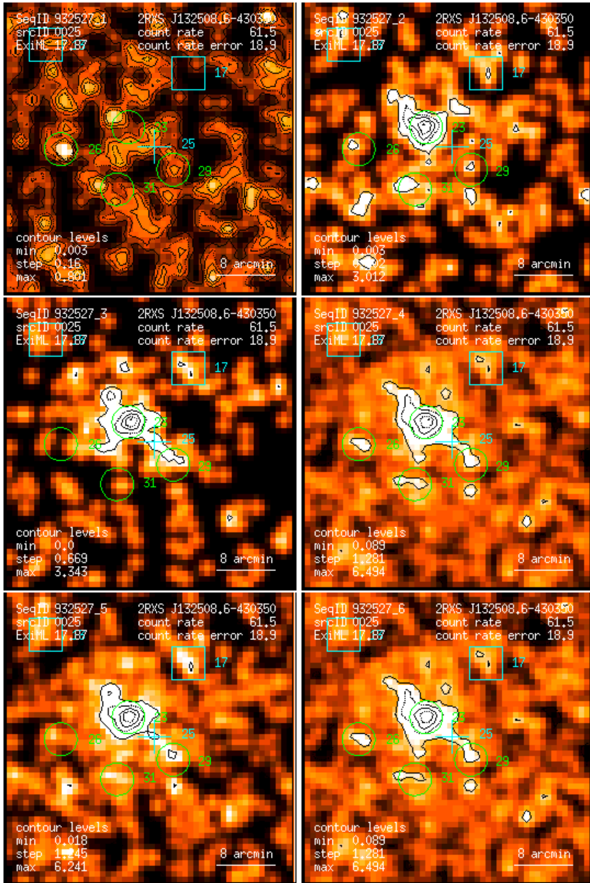
Figure 25: RASS 932527: detection 0025: band rate images, Gaussian filter: (1) PSPC channels 11 – 41, (2) 52 – 90, (3) 91 – 201, (4) 11 – 235, (5) 52 – 201, (6) 11 – 201. Broad band rates in counts/ks. Band rate contour levels in counts/ks/arcmin 2 .
