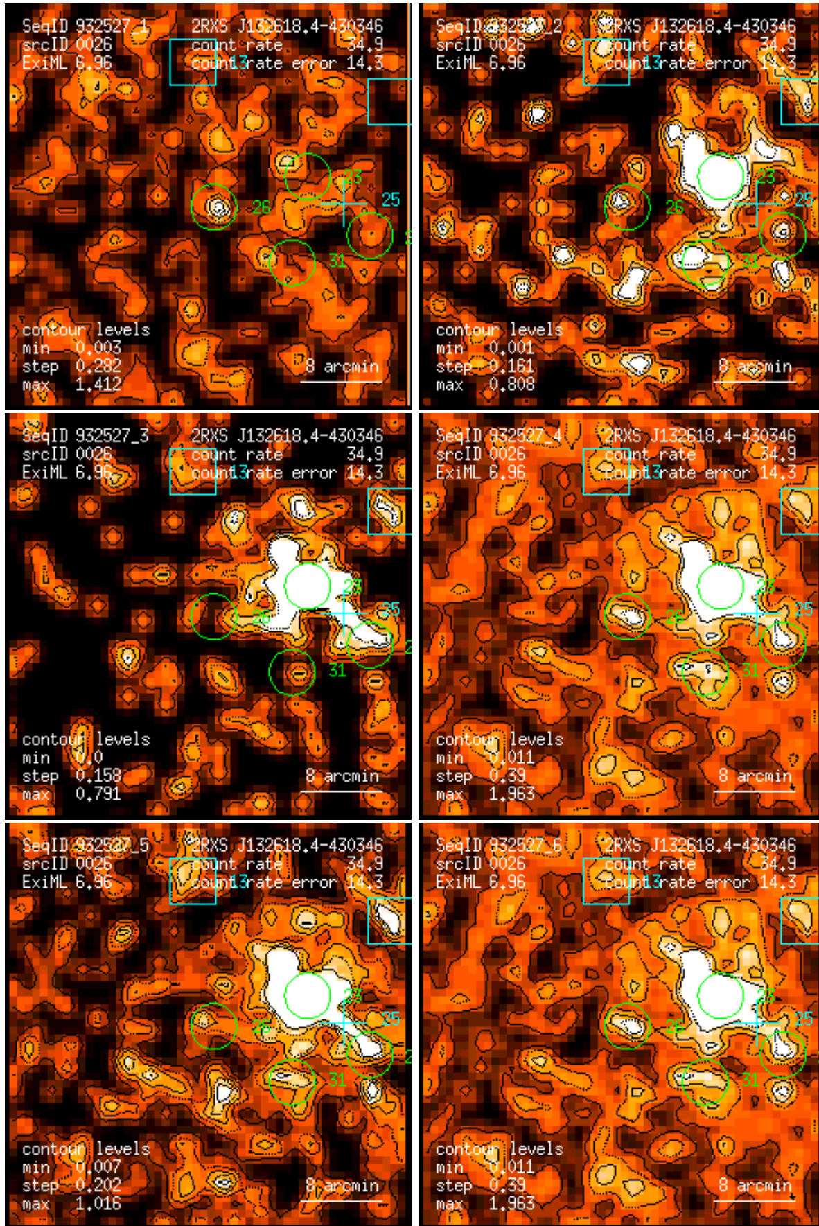
Figure 26: RASS 932527: detection 0026: band rate images, Gaussian filter: (1) PSPC channels 11 – 41, (2) 52 – 90, (3) 91 – 201, (4) 11 – 235, (5) 52 – 201, (6) 11 – 201. Broad band rates in counts/ks. Band rate contour levels in counts/ks/arcmin 2 .
