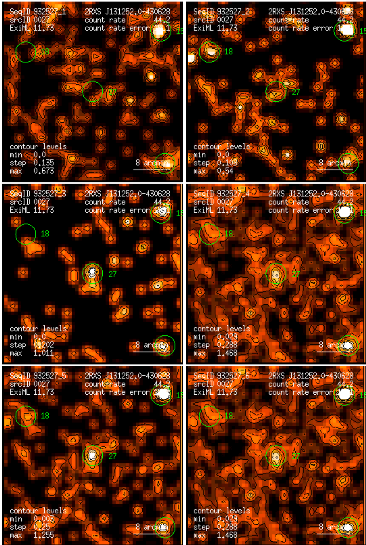
Figure 27: RASS 932527: detection 0027: band rate images, Gaussian filter: (1) PSPC channels 11 – 41, (2) 52 – 90, (3) 91 – 201, (4) 11 – 235, (5) 52 – 201, (6) 11 – 201. Broad band rates in counts/ks. Band rate contour levels in counts/ks/arcmin 2 .
