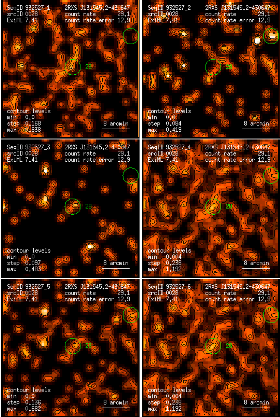
Figure 28: RASS 932527: detection 0028: band rate images, Gaussian filter: (1) PSPC channels 11 – 41, (2) 52 – 90, (3) 91 – 201, (4) 11 – 235, (5) 52 – 201, (6) 11 – 201. Broad band rates in counts/ks. Band rate contour levels in counts/ks/arcmin 2 .
