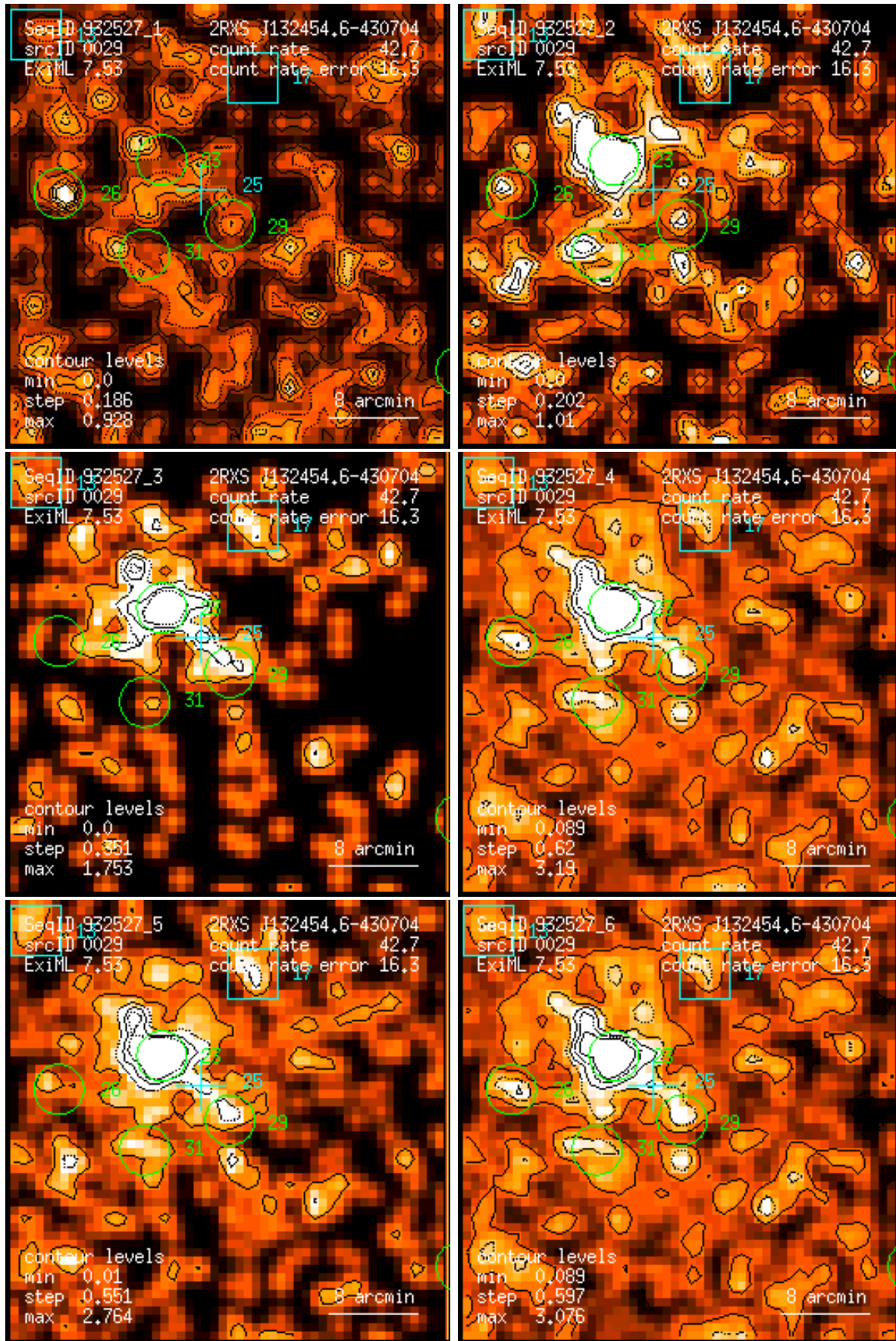
Figure 29: RASS 932527: detection 0029: band rate images, Gaussian filter: (1) PSPC channels 11 – 41, (2) 52 – 90, (3) 91 – 201, (4) 11 – 235, (5) 52 – 201, (6) 11 – 201. Broad band rates in counts/ks. Band rate contour levels in counts/ks/arcmin 2 .
