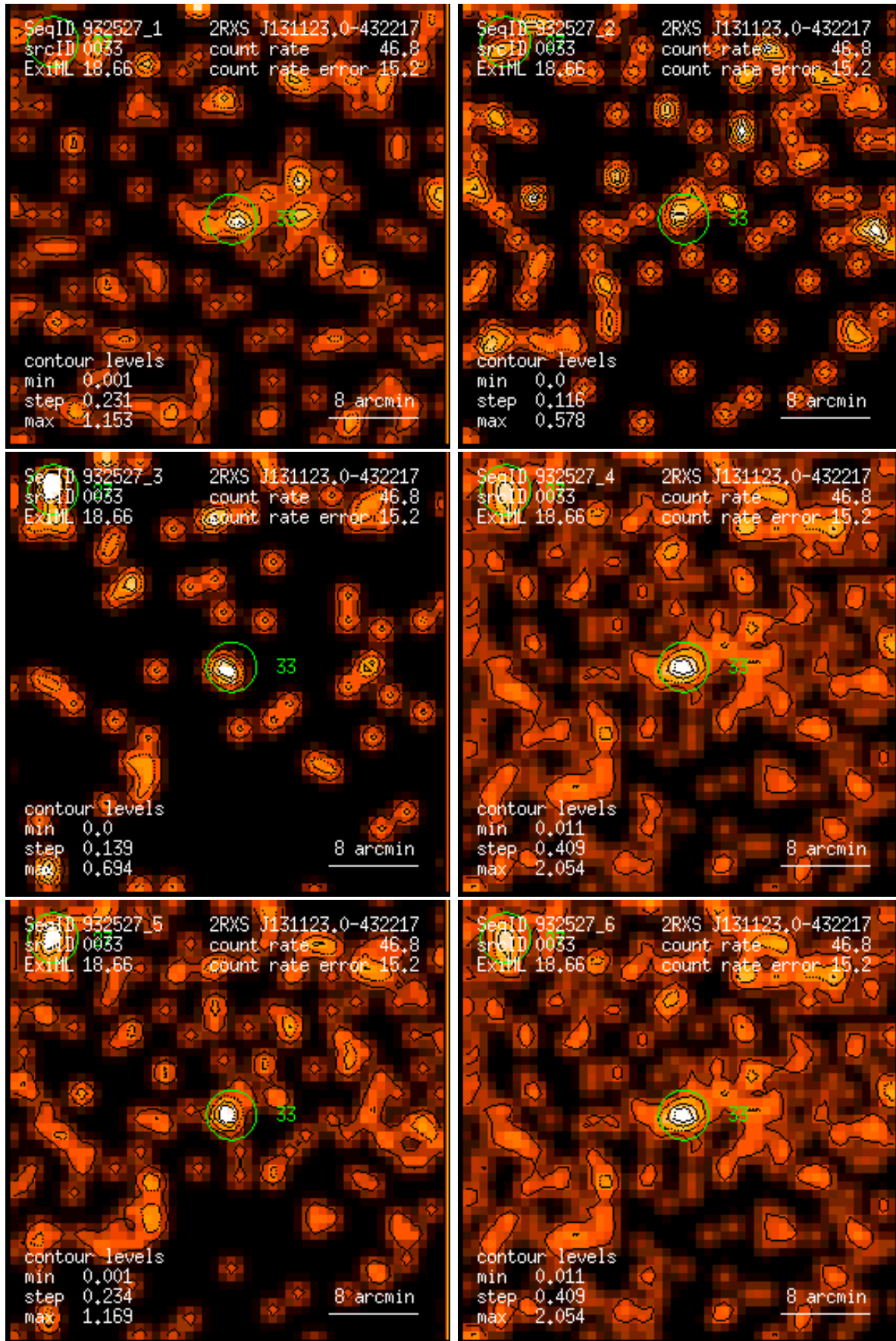
Figure 33: RASS 932527: detection 0033: band rate images, Gaussian filter: (1) PSPC channels 11 – 41, (2) 52 – 90, (3) 91 – 201, (4) 11 – 235, (5) 52 – 201, (6) 11 – 201. Broad band rates in counts/ks. Band rate contour levels in counts/ks/arcmin 2 .
